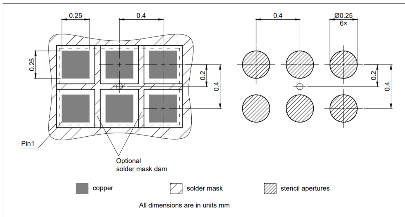
Figure 4: Footprint Recommendation
