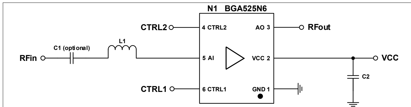
Figure 2: BGA525N6 Application Schematic for L1/L2/L5
