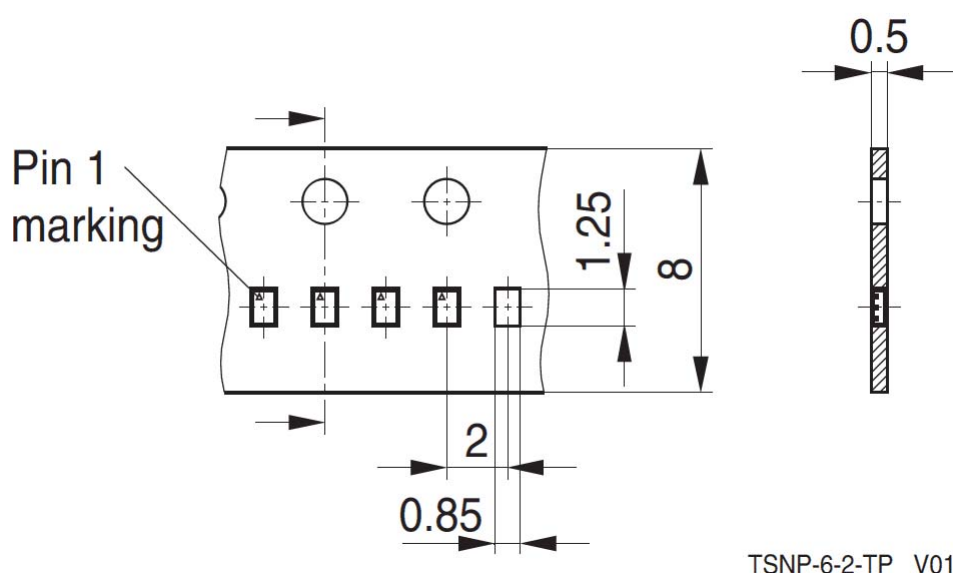
Figure 11 Tape & Reel Dimensions TSNP-6-2 (reel diameter 180 mm, pieces/reel 15000)
