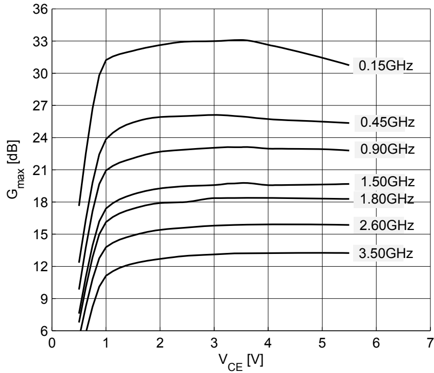
Figure 10 Maximum power gain G_{\max} = f(V_{CE}) , I_C = 250 mA, f = parameter
