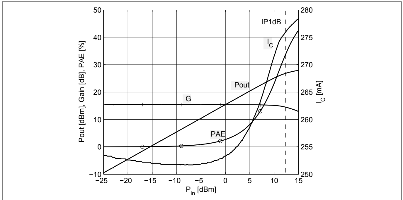
Figure 22 P_{out} , G , I_C , PAE = f(P_{in}) , V_{CE} = 5\text{ V} , I_{Cq} = 250\text{ mA} , f = 2.6\text{ GHz} , Z_L = Z_{L,opt}(P_{out})
