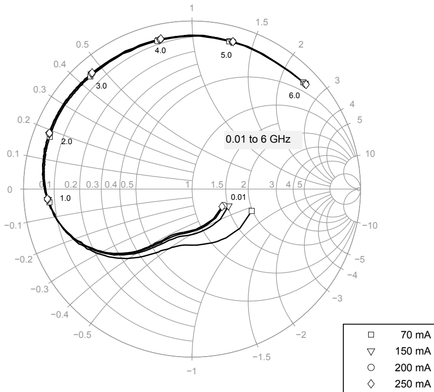
Figure 11 Input reflection coefficient S_{11} = f(f) , V_{CE} = 5 V, I_C = parameter
