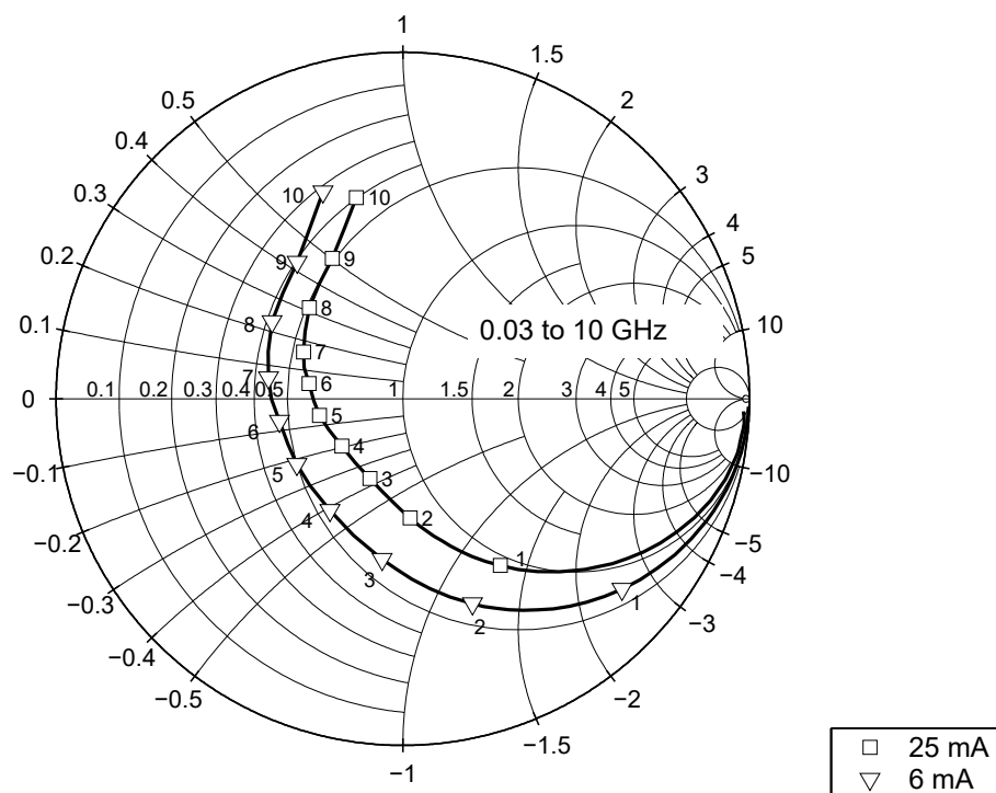
Figure 16 Output reflection coefficient S_{22} = f(f) , V_{CE} = 3 \text{ V} , I_C = 6 / 25 \text{ mA}
