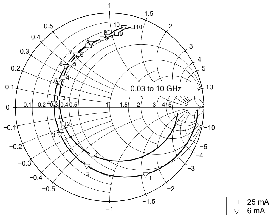
Figure 14 Input reflection coefficient S_{11} = f(f) , V_{CE} = 3 V, I_C = 6 / 25 mA
