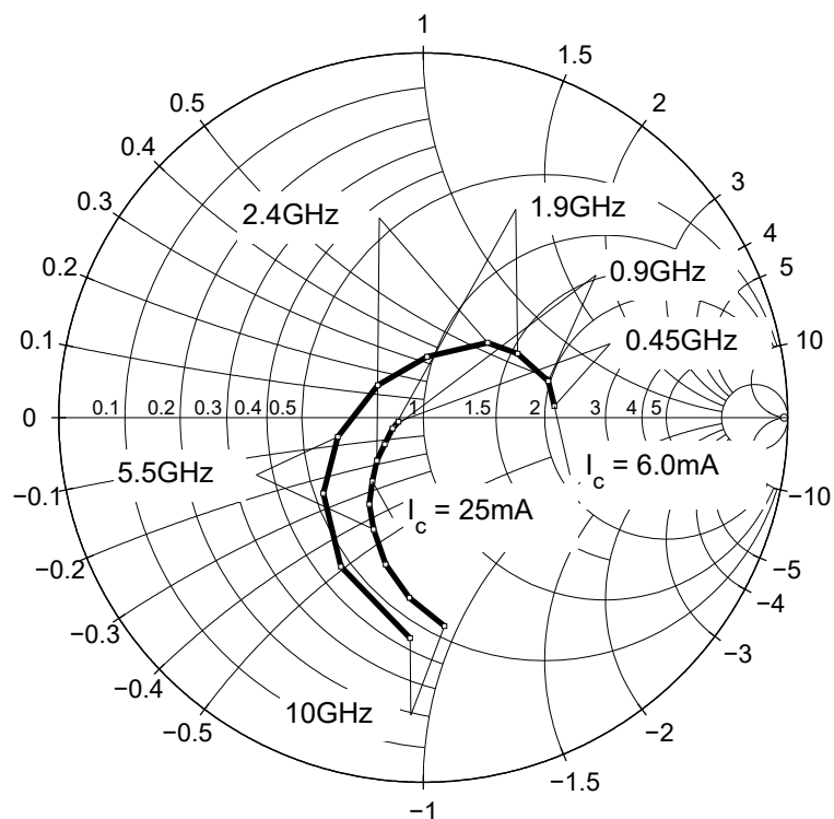
Figure 15 Source impedance for minimum noise figure Z_{opt} = f(f) , V_{CE} = 3 V, I_C = 6 / 25 mA
