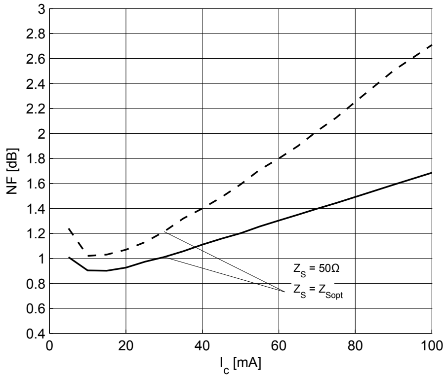
Figure 20 Noise figure NF_{50} = f(I_C) , Z_S = 50 \Omega , NF_{min} = f(I_C) , Z_S = Z_{S,opt} , V_{CE} = 3 \text{ V} , f = 2.4 \text{ GHz}
