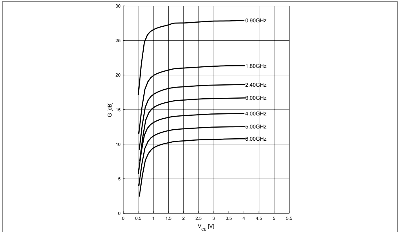
Figure 7 Maximum power gain G_{\max} = f(V_{CE}) , I_C = 80 mA, f = parameter in GHz
