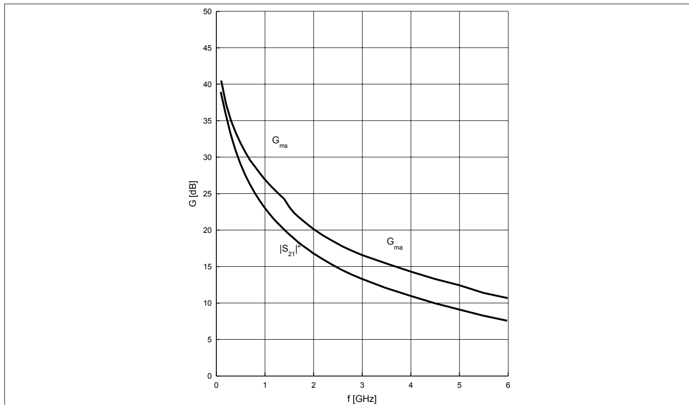
Figure 5 Gain G_{ma} , G_{ms} , |S_{21}|^2 = f(f) , V_{CE} = 3 V, I_C = 80 mA
