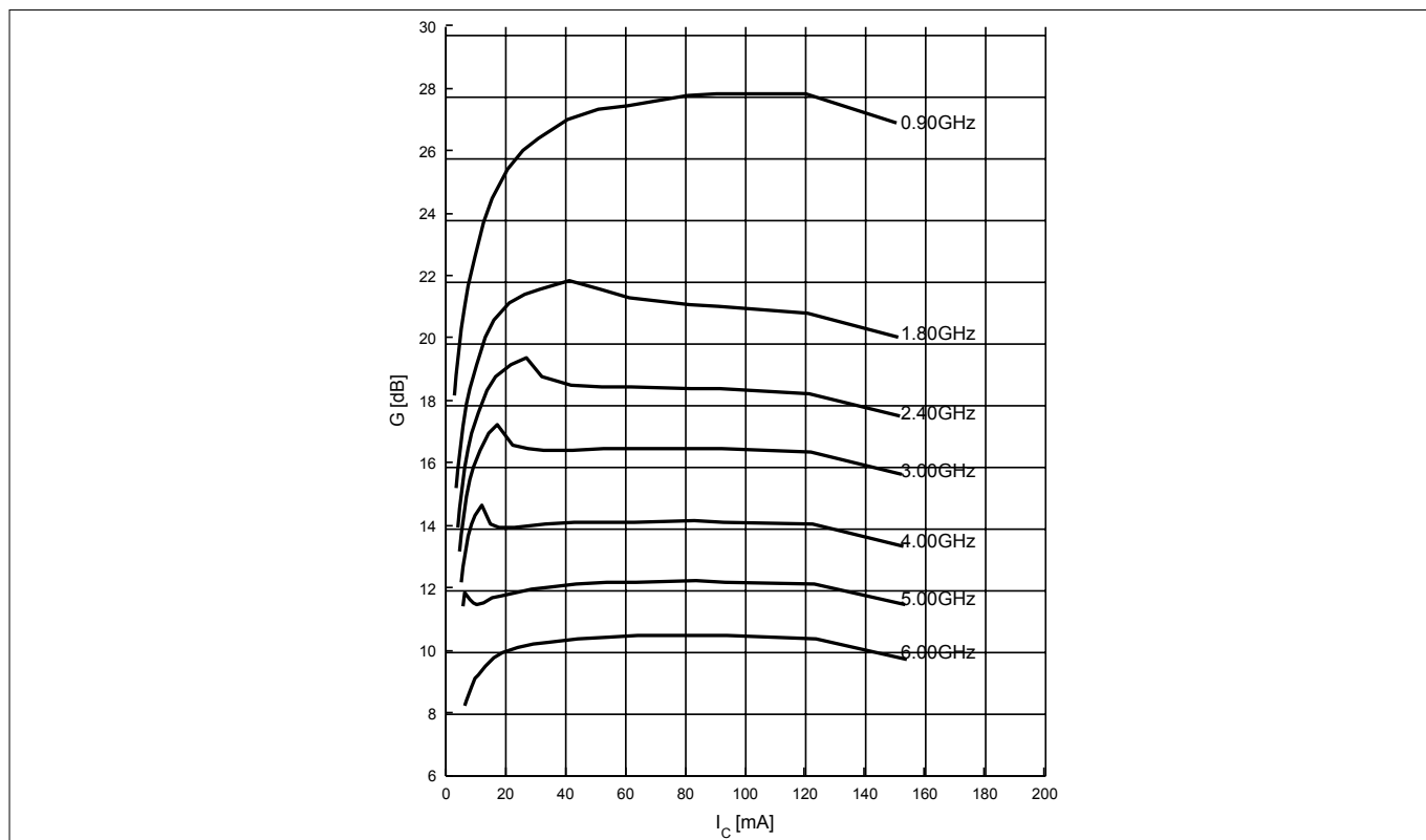
Figure 6 Maximum power gain G_{max} = f(I_C) , V_{CE} = 3 V, f = parameter in GHz
