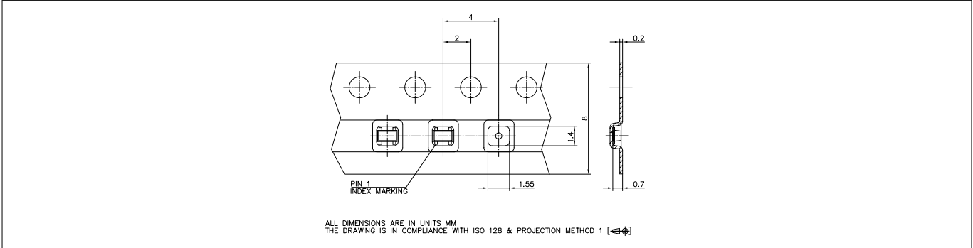
Figure 6 Tape dimensions
