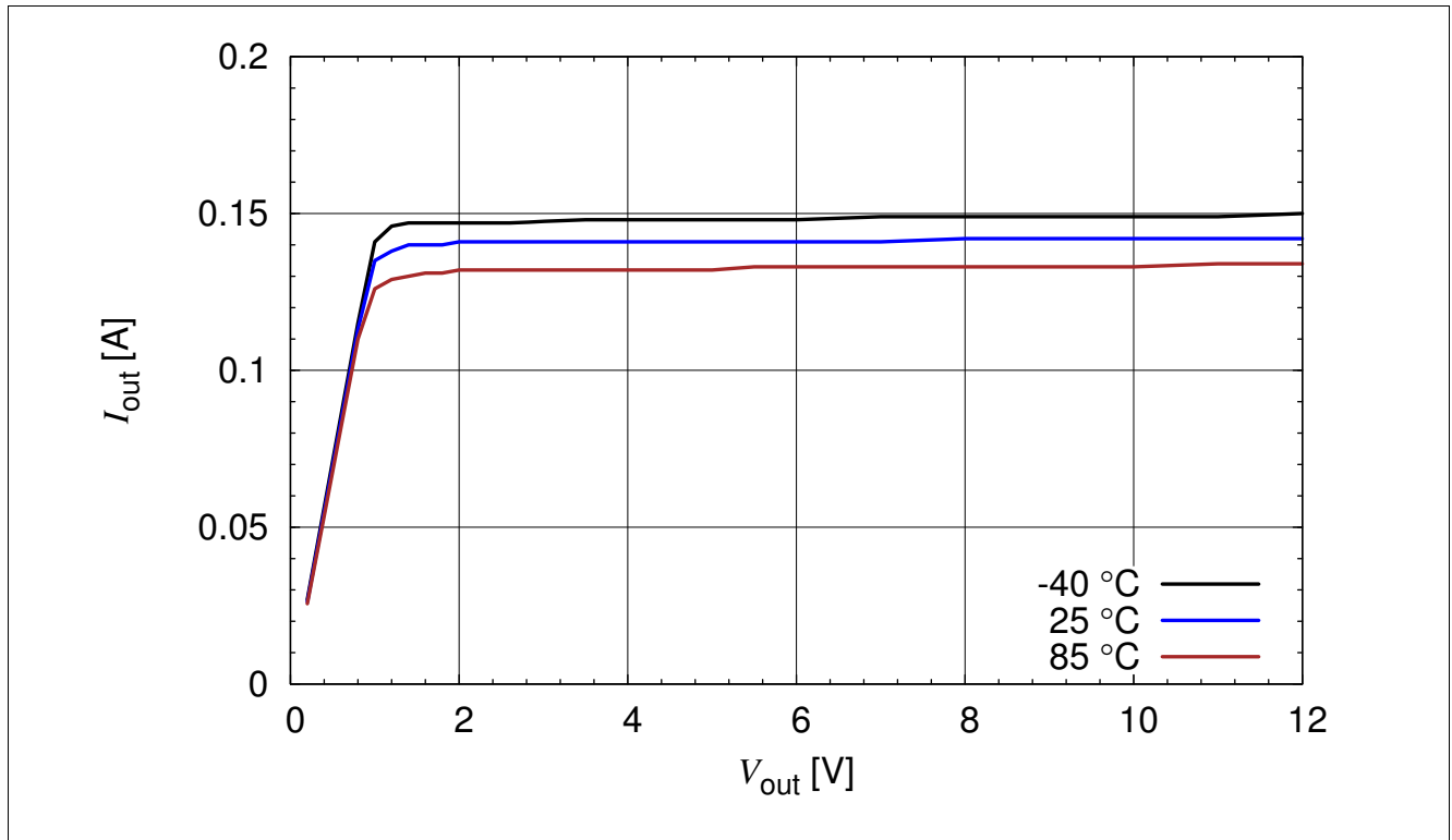
Figure 3-8 BCR 420U: Output Current versus V_{out} I_{out} = f(V_{out}) , V_{EN} = 40 V, R_{ext} = 6 \Omega , T_A = \text{Parameter}
