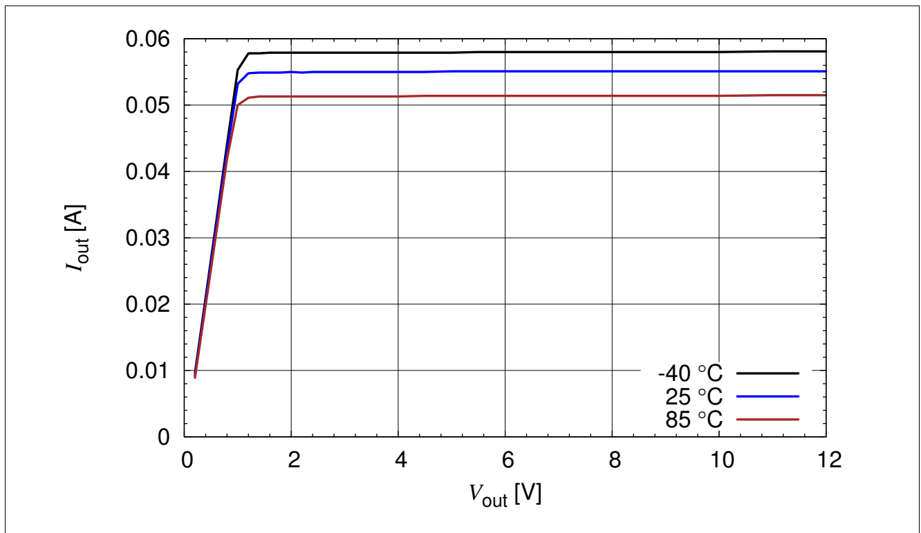
Figure 3-7 BCR 420U: Output Current versus V_{out} I_{out} = f(V_{out}) , V_{EN} = 40 V, R_{ext} = 20 \Omega , T_A = \text{Parameter}
