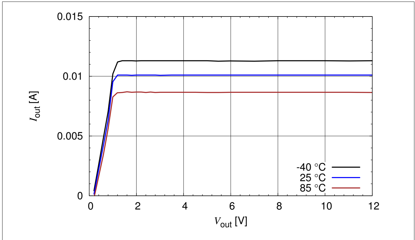
Figure 3-6 BCR 420U: Output Current versus V_{out} I_{out} = f(V_{out}) , V_{EN} = 40 V, R_{ext} = \text{open} , T_A = \text{Parameter}
