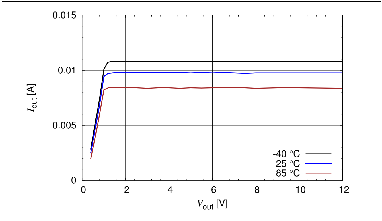
Figure 3-16 BCR 421U: Output Current versus V_{out} I_{out} = f(V_{out}) , V_{EN} = 3.3 V, R_{ext} = \text{open} , T_A = \text{Parameter}
