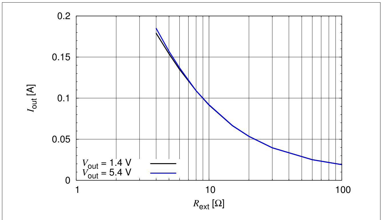
Figure 3-15 BCR 421U: Output Current versus R_{ext} I_{out} = f(R_{ext}) , V_{EN} = 3.3 V, V_{out} = \text{Parameter}
