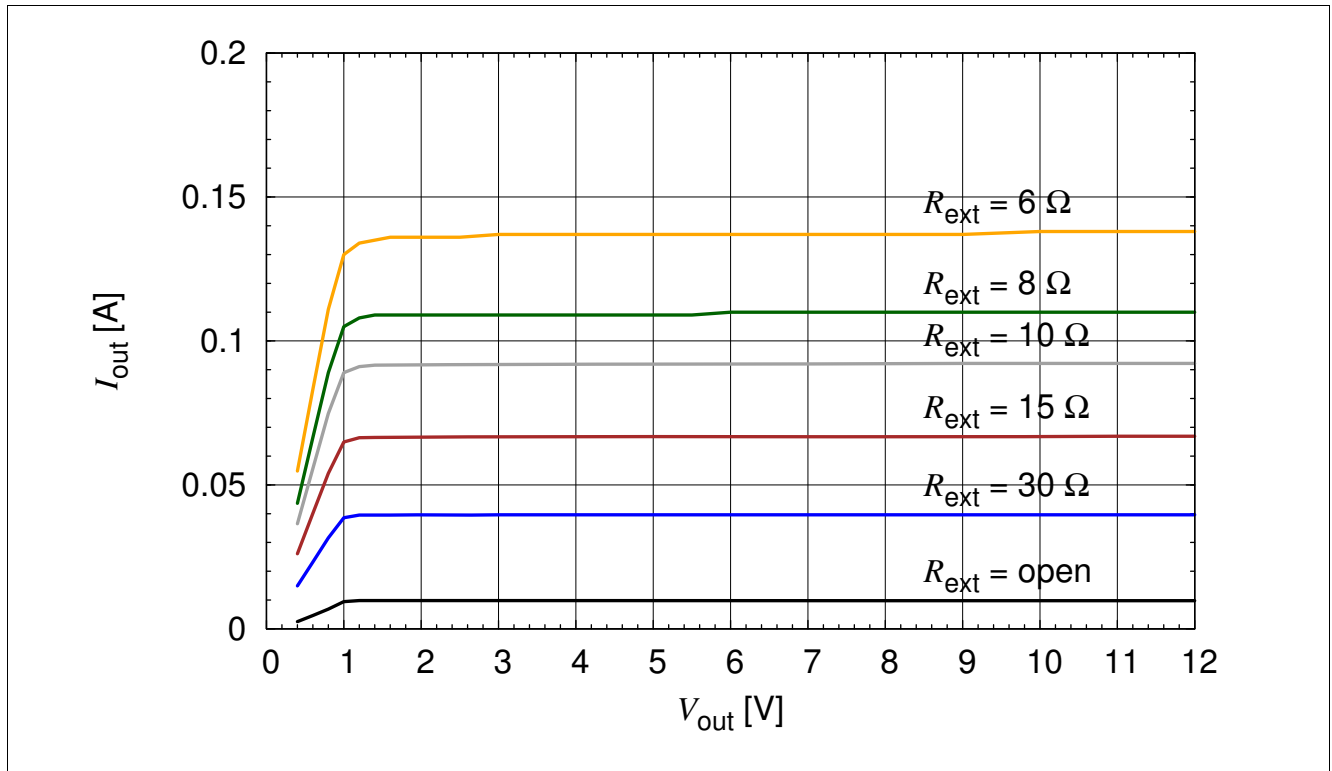
Figure 3-14 BCR 421U: Output Current versus V_{out} I_{out} = f(V_{out}) , V_{EN} = 3.3 V, R_{ext} = \text{Parameter}
