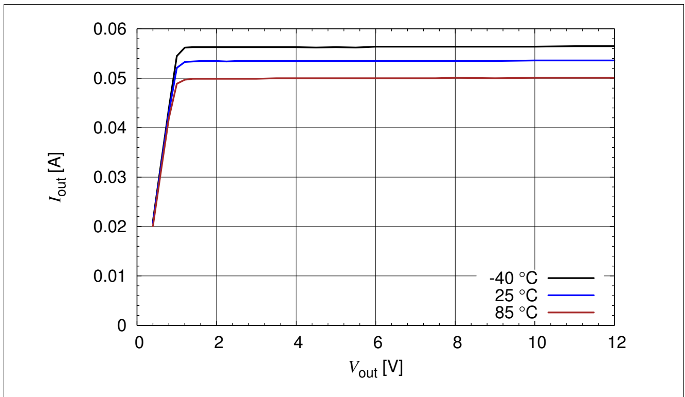
Figure 3-17 BCR 421U: Output Current versus V_{out} I_{out} = f(V_{out}) , V_{EN} = 3.3 V, R_{ext} = 20 \Omega , T_A = \text{Parameter}
