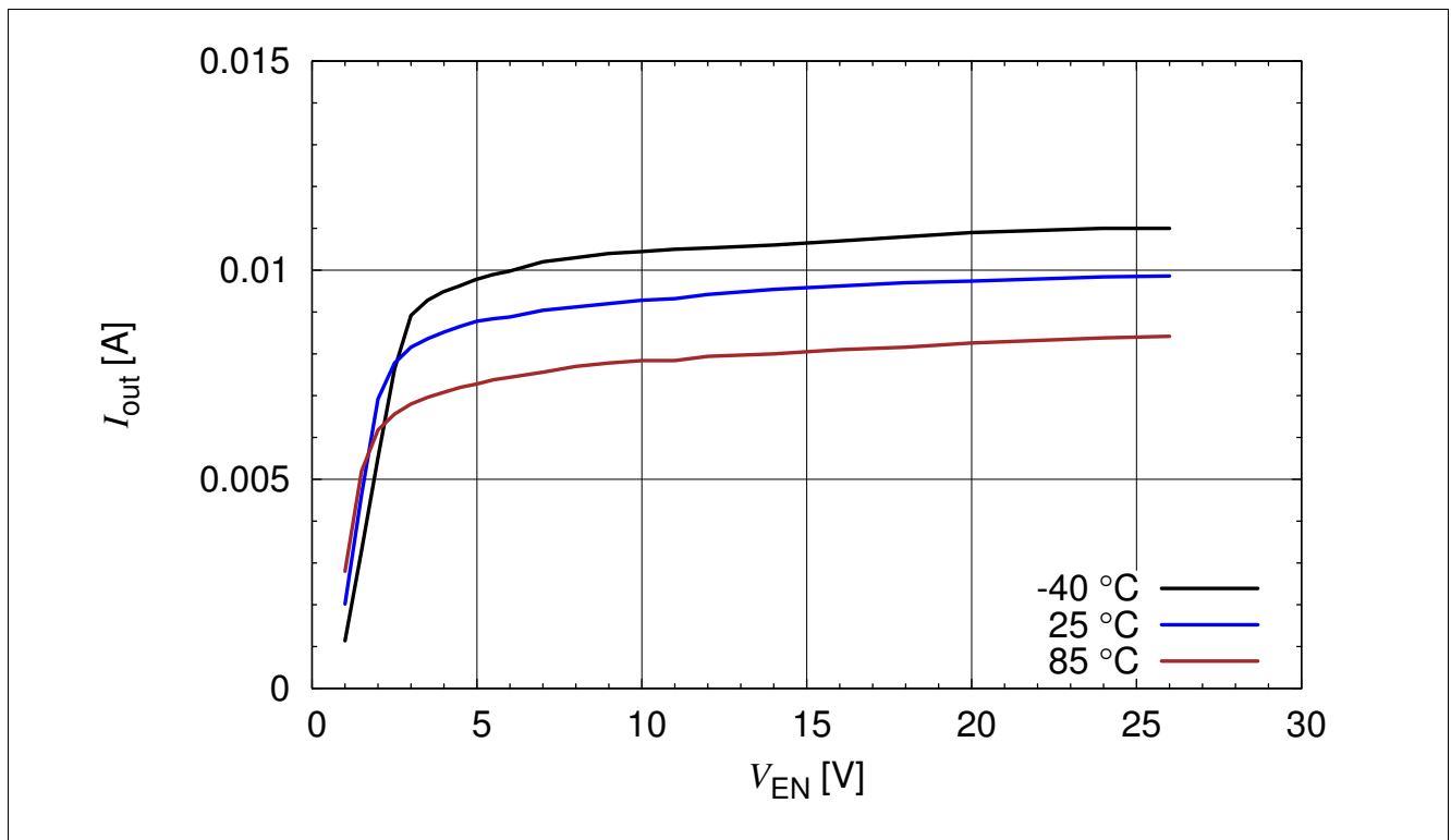
Figure 3-9 BCR 420U: Output Current versus V_{EN} I_{out} = f(V_{EN}) , V_{out} = 2 V, R_{ext} = \text{open} , T_A = \text{Parameter}
