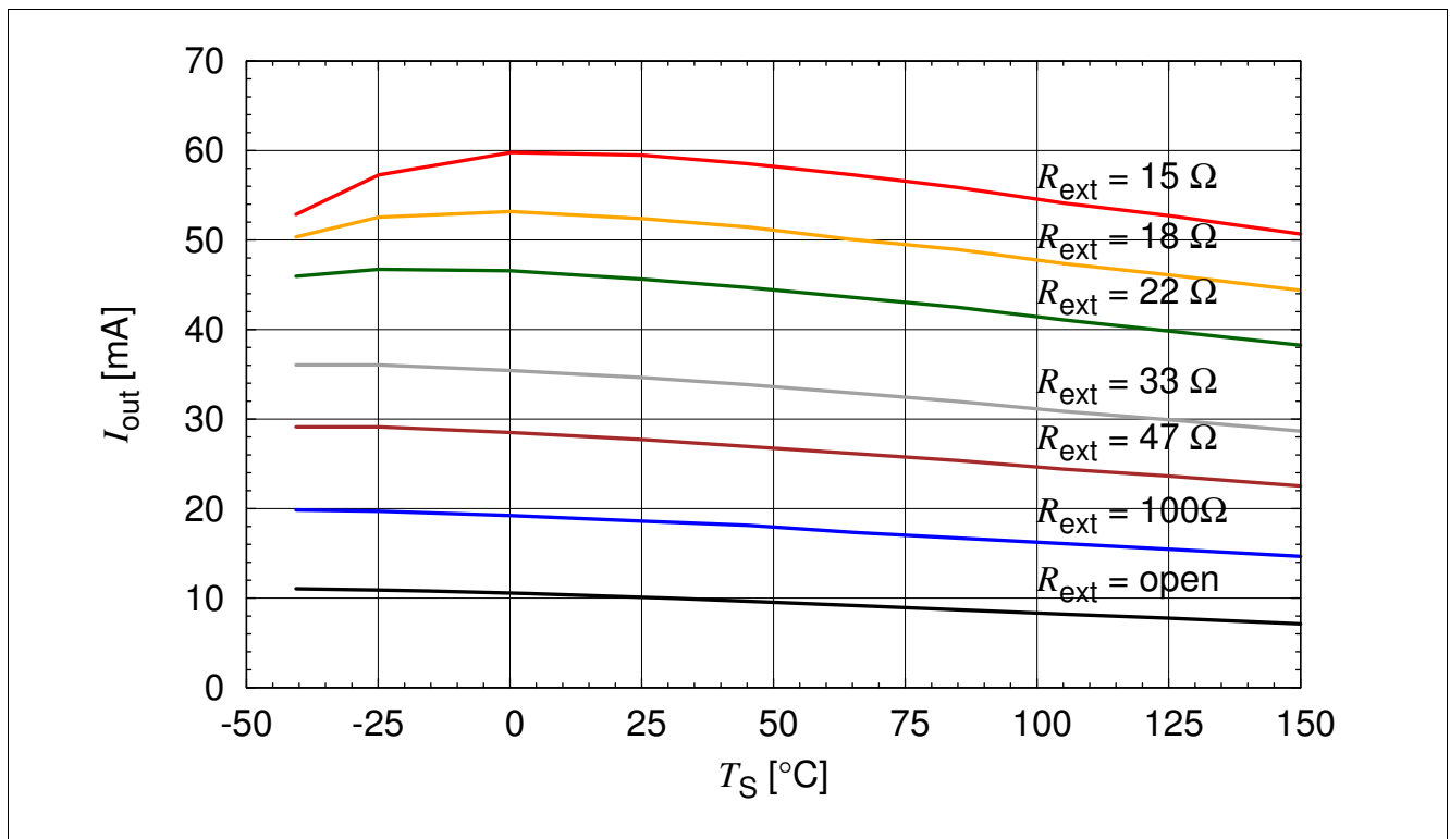
Figure 3-9 Output Current versus T_S I_{\text{out}} = f(T_S) , V_S = 10 \text{ V} , V_S - V_{\text{out}} = 1.4 \text{ V} , R_{\text{ext}} = \text{Parameter}
