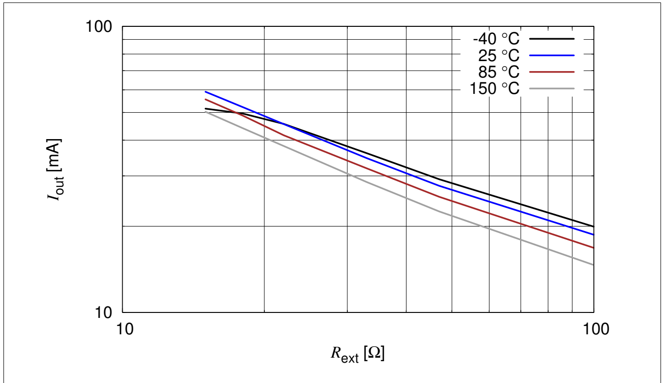
Figure 3-8 Output Current versus R_{\text{ext}} I_{\text{out}} = f(R_{\text{ext}}) , V_S = 10 \text{ V} , V_S - V_{\text{out}} = 1.4 \text{ V} , T_A = \text{Parameter}
