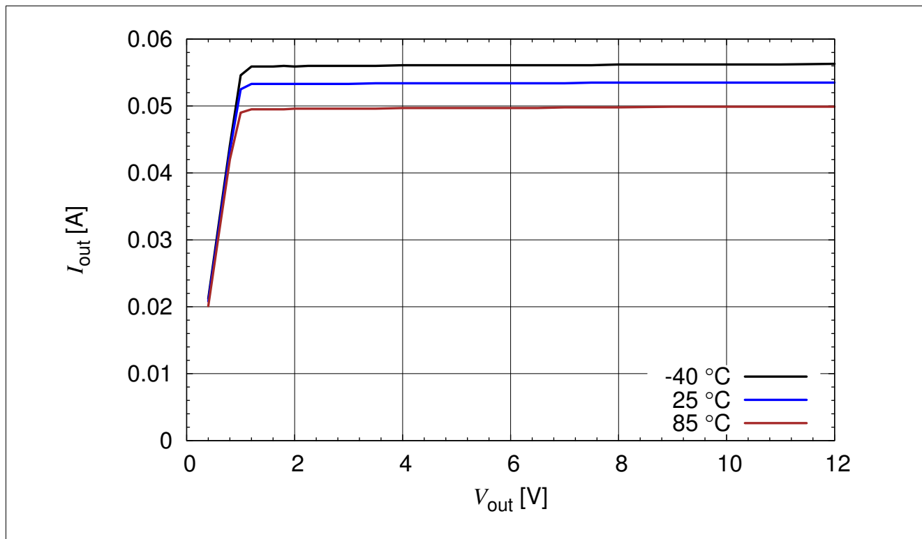
Figure 3-17 BCR 321U: Output Current versus V_{out} I_{out} = f(V_{out}) , V_{EN} = 3.3 V, R_{ext} = 20 Ω, T_A = \text{Parameter}
