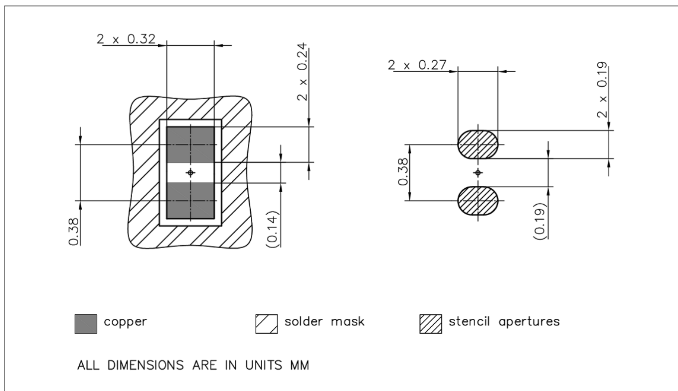
Figure 12 Foot print
