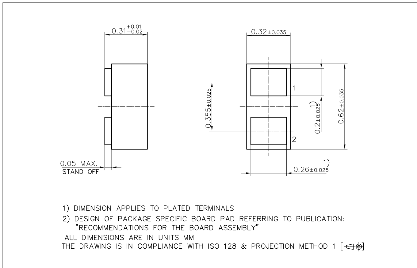
Figure 11 Package outline
