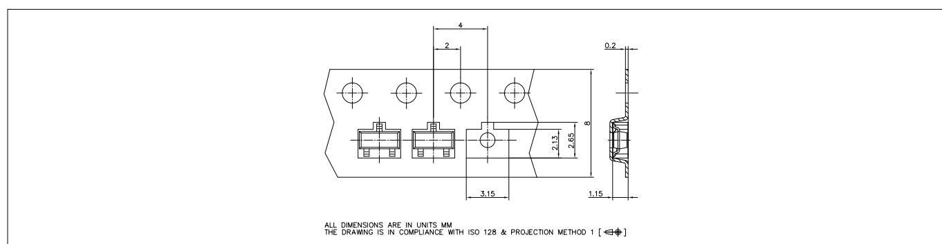
Figure 10 Tape dimensions
