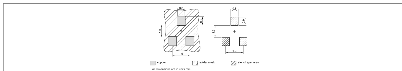
Figure 8 Foot print
