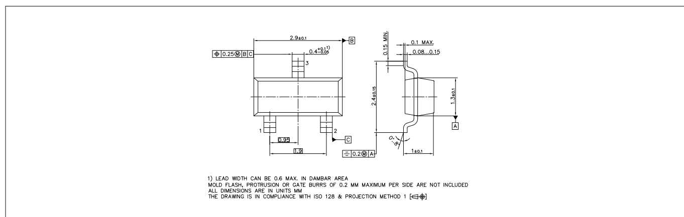
Figure 7 Package outline
