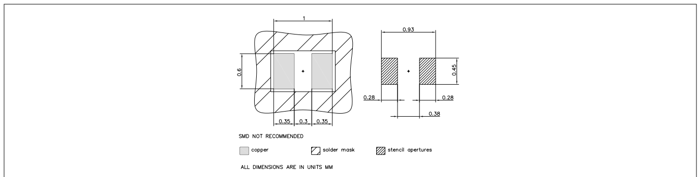
Figure 12 Foot print
