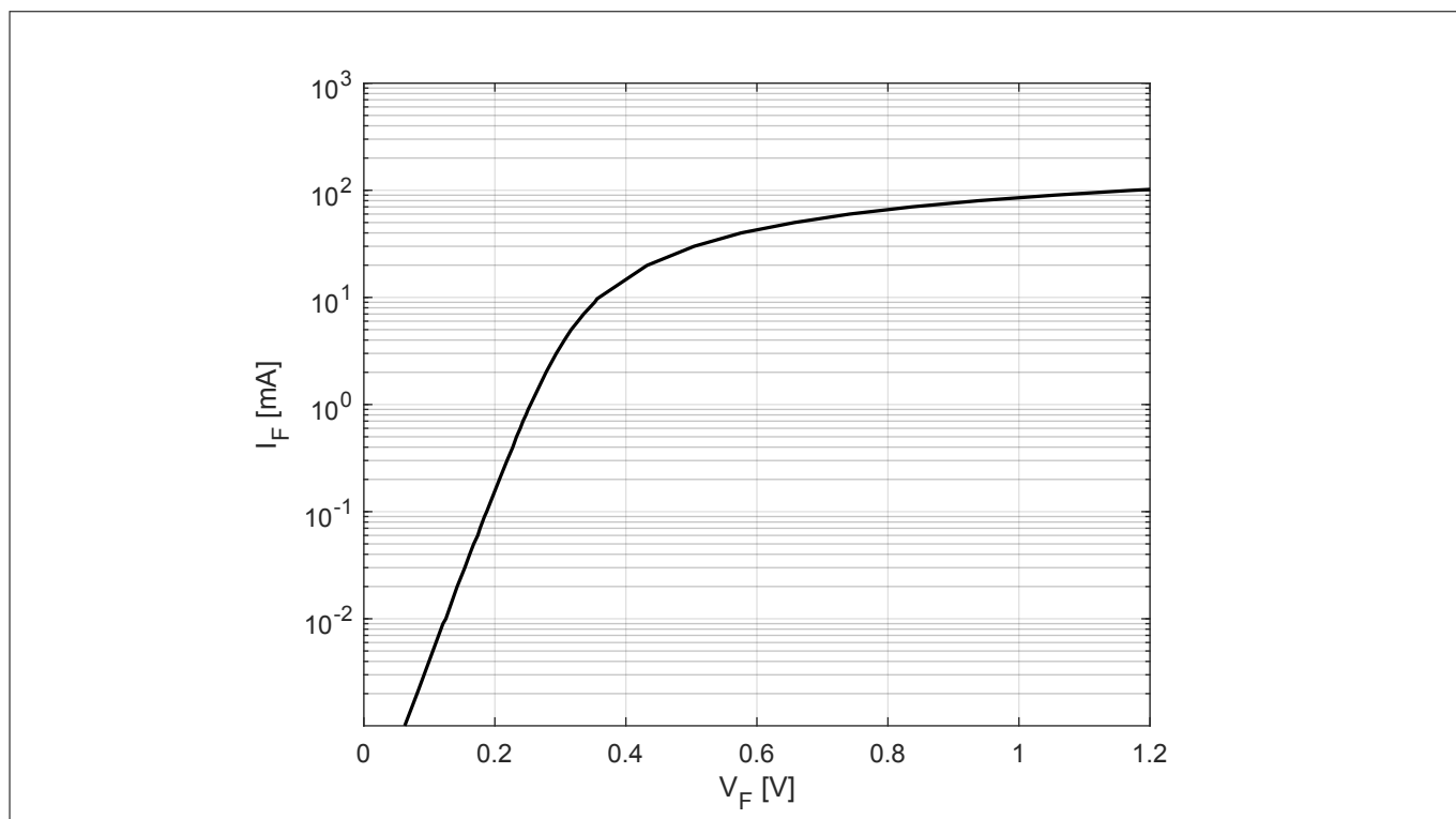
Figure 3 Forward current I_F vs. forward voltage V_F
