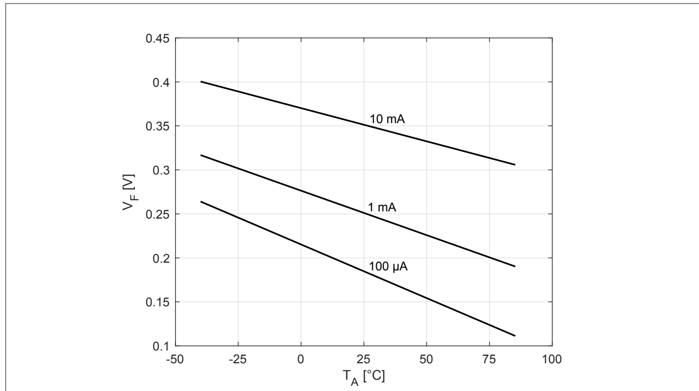
Figure 4 Forward voltage V_F vs. ambient temperature T_A at forward currents I_F = 100 \mu A, 1 mA and 10 mA
