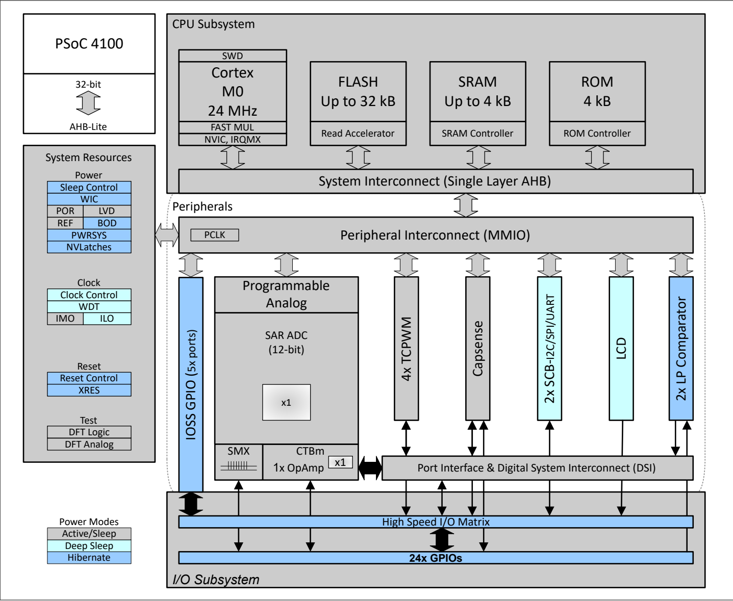
Figure 1 Block diagram
