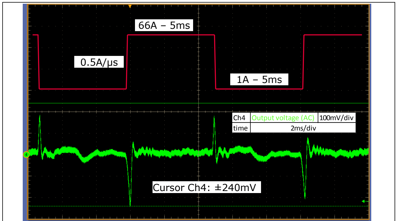
Figure 15 Output voltage response to 1 A to 66 A dynamic load steps with 0.5 A/ \mu s current slope every 5 ms
