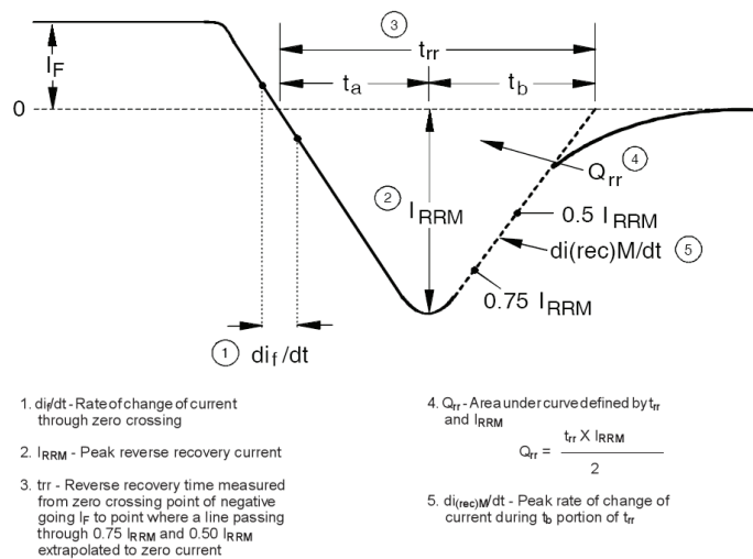
Fig. WF3 - Reverse Recovery Waveform and Definitions
