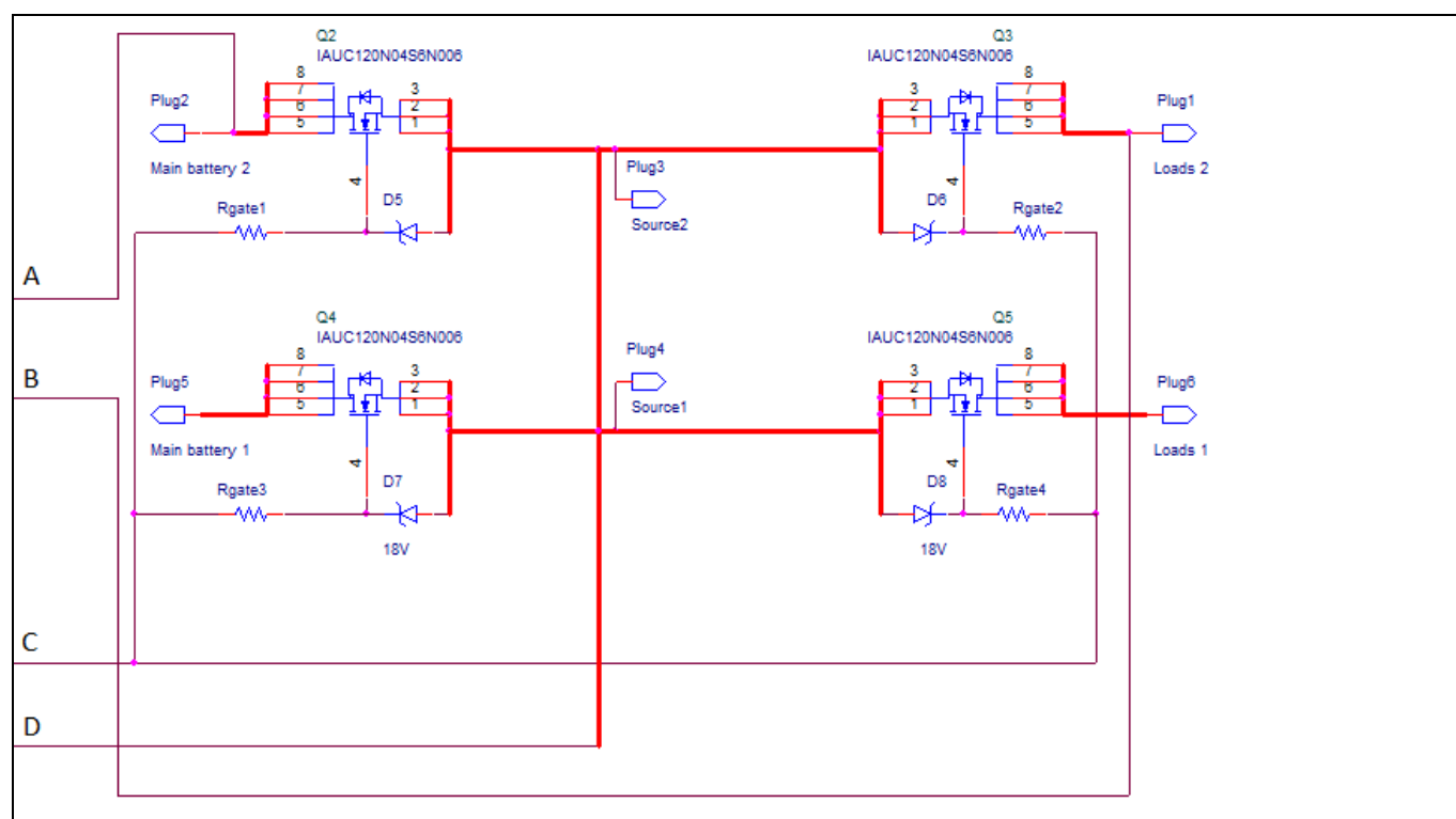
Figure 7 Power side, valid for both AUIR3241S and AUIR3242S
