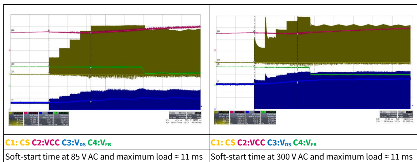
Figure 19 Soft-start
