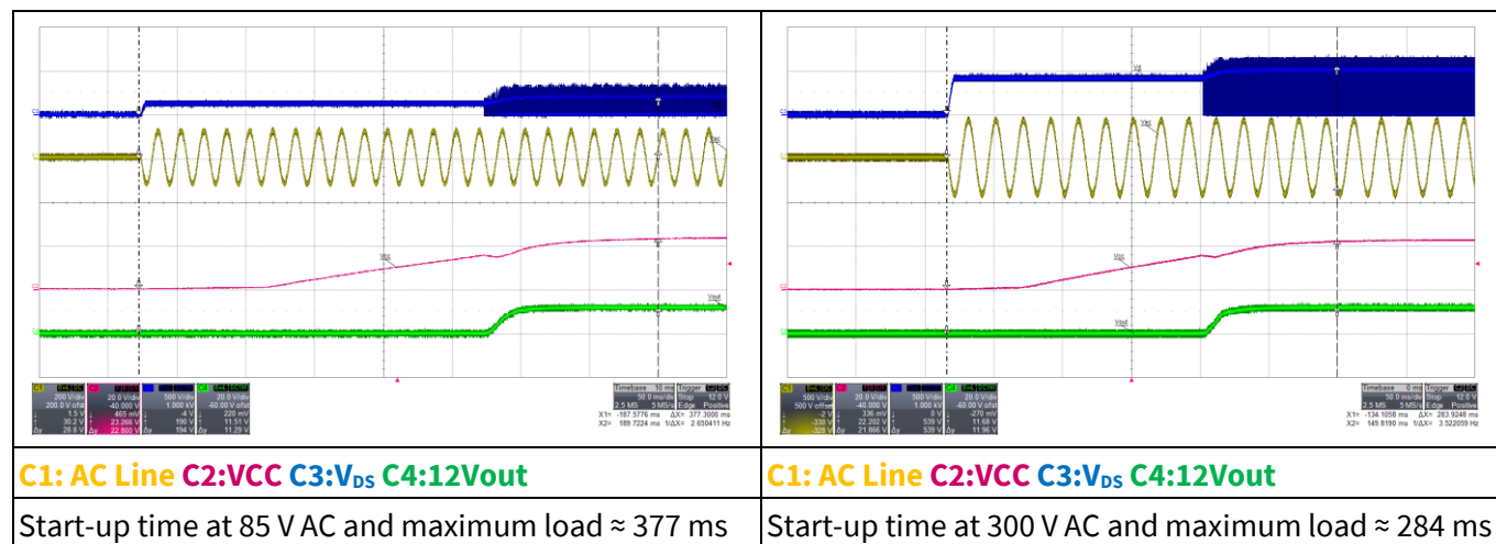
Figure 18 Start-up
