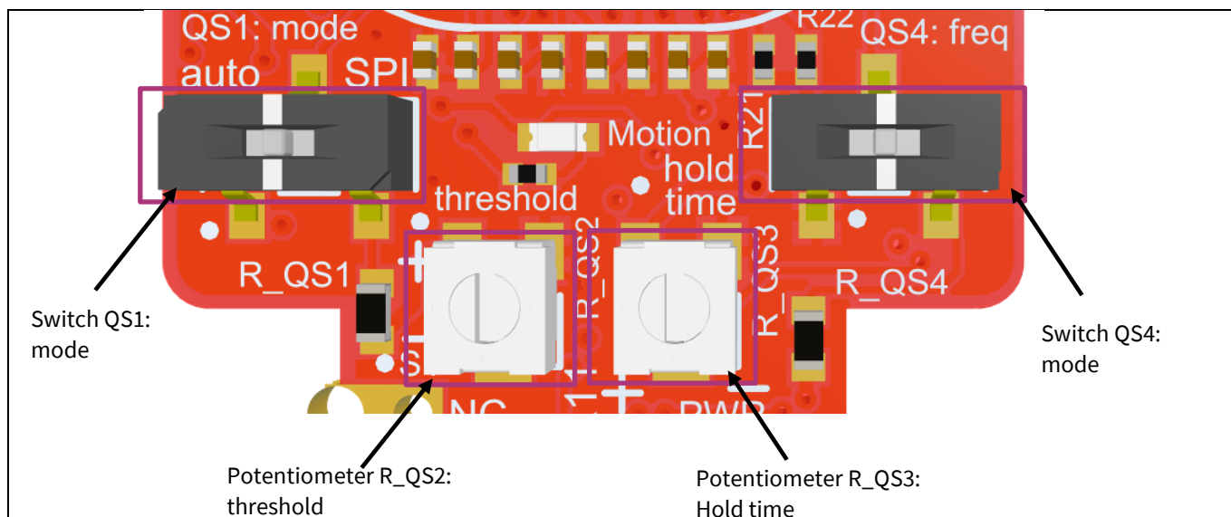
Figure 13 Overview of QS1 to QS4 signals on the BGT60LTR11AIP Radar Shield2Go from the top
