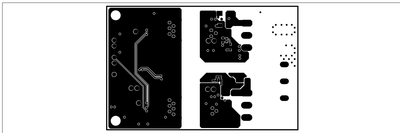
Figure 14 PCB bottom layer
