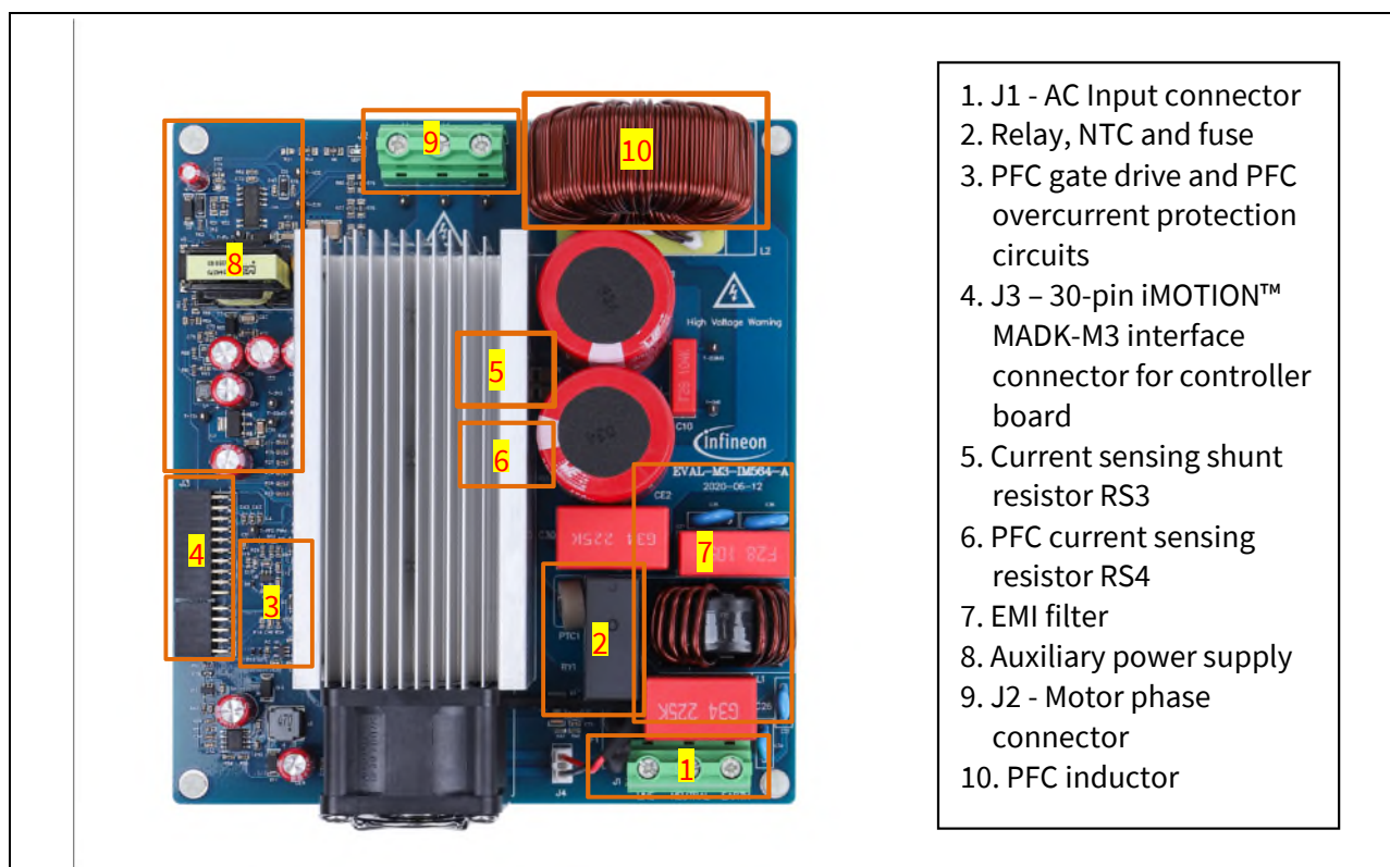
Figure 2 Functional groups of the EVAL-M3-IM564 evaluation board's top side
