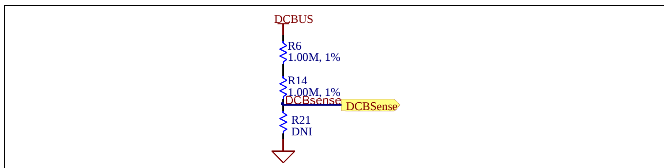
Figure 19 DC bus sense resistor on EVAL-M3-IM564 evaluation board
