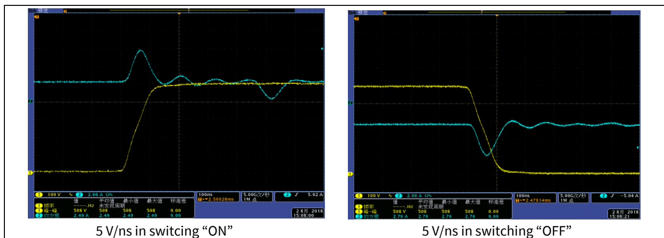
Figure 33 Typical dv/dt test waveform. It is IM818-MCC work on 380 V AC input at switching current is 2A.
