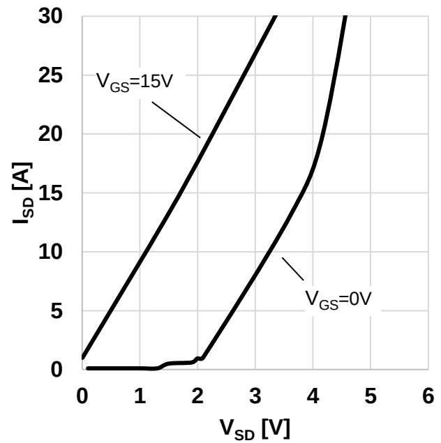
Figure 14 Typical body diode forward current as function of forward voltage, V_{GS} as parameter ( I_{SD} = f(V_{DS}) , T_{vj} = 175^{\circ}\text{C} , t_p = 20\mu\text{s} )
