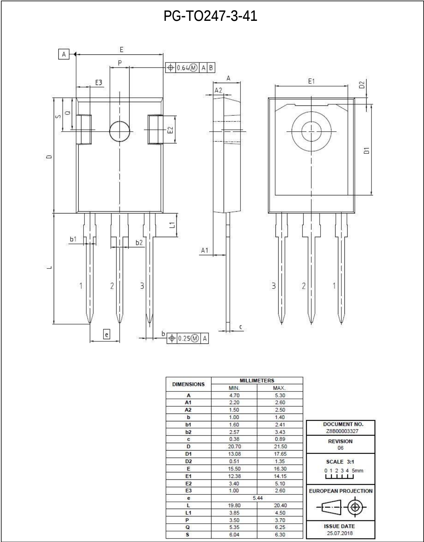
Figure 22 Package drawing
