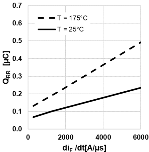
Figure 19 Typical reverse recovery charge as a function of diode current slope (Q_{rr} = f(di_F/dt), V_{DD} = 800V, V_{GS} = 0V/18V, I_D = 13A, \text{ind. load, test circuit in Fig. E, body diode at } V_{GS} = 0V)
