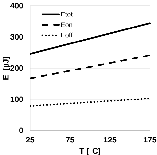
Figure 15 Typical switching energy losses as a function of junction temperature ( E = f(T_{vj}) , V_{DD} = 800\text{V} , V_{GS} = 0\text{V}/18\text{V} , R_{G,ext} = 2\Omega , I_D = 13\text{A} , ind. load, test circuit in Fig. E, diode: body diode at V_{GS} = 0\text{V} )
