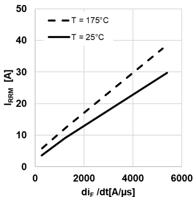
Figure 20 Typical reverse recovery current as a function of diode current slope (I_{rrm} = f(di_F/dt), V_{DD} = 800V, V_{GS} = 0V/18V, I_D = 25A, \text{ind. load, test circuit in Fig. E, body diode at } V_{GS} = 0V)
