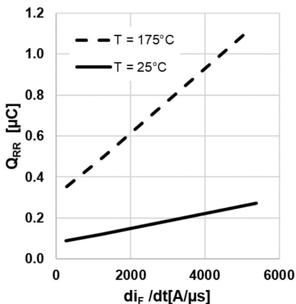
Figure 19 Typical reverse recovery charge as a function of diode current slope (Q_{rr} = f(di_F/dt), V_{DD} = 800V, V_{GS} = 0V/18V, I_D = 25A, \text{ind. load, test circuit in Fig. E, body diode at } V_{GS} = 0V)
