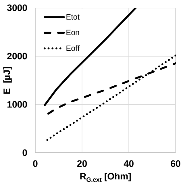
Figure 17 Typical switching energy losses as a function of gate resistance (E = f(R_{G,ext}), V_{DD} = 800V, V_{GS} = 0V/18V, I_D = 25A, T_{vj} = 175^\circ C, \text{ind. load, test circuit in Fig. E, diode: body diode at } V_{GS} = 0V)
