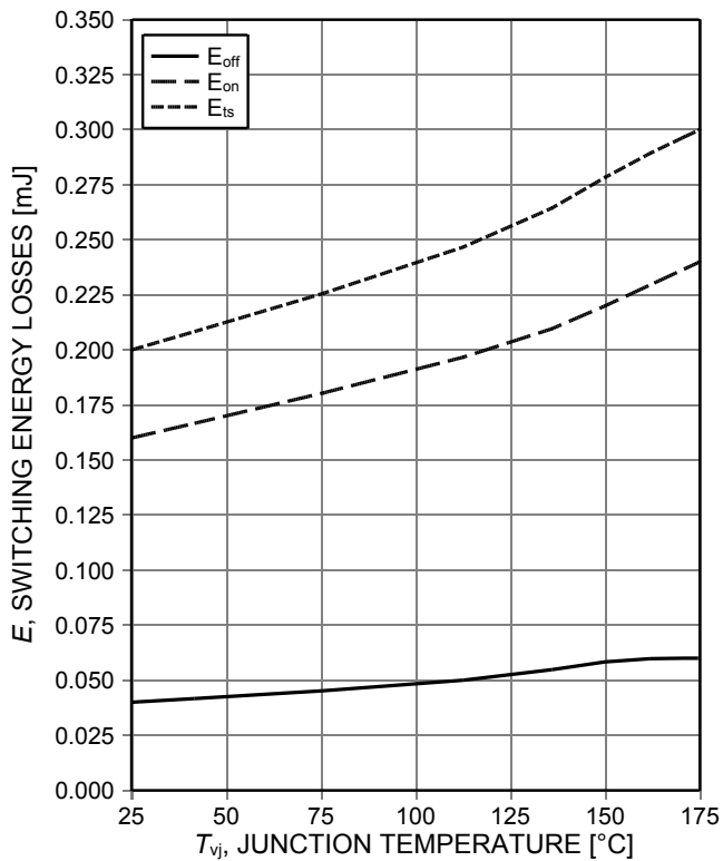
Figure 13. Typical switching energy losses as a function of junction temperature (inductive load, V_{CE}=400V , V_{GE}=15/0V , I_C=7.5A , r_G=39\Omega , Dynamic test circuit in Figure E)
