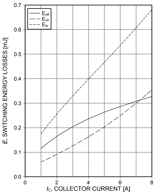
Figure 11. Typical switching energy losses as a function of collector current (inductive load, T_{vj}=175^\circ C , V_{CE}=400V , V_{GE}=15/0V , r_G=43\Omega , Dynamic test circuit in Figure E)
