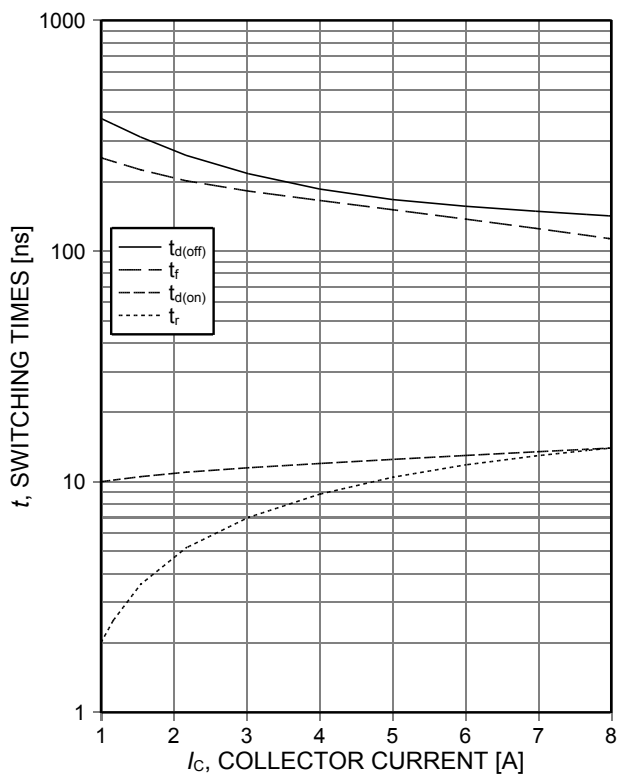
Figure 7. Typical switching times as a function of collector current (inductive load, T_{vj}=175^{\circ}C , V_{CE}=400V , V_{GE}=15/0V , r_G=43\Omega , Dynamic test circuit in Figure E)
