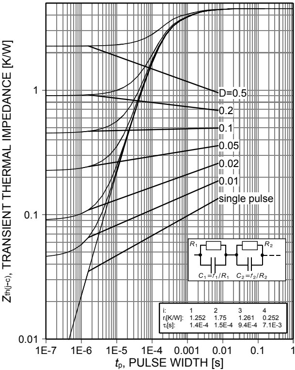
Figure 20. Diode transient thermal impedance as a function of pulse width 1) ( D = t_p/T )
