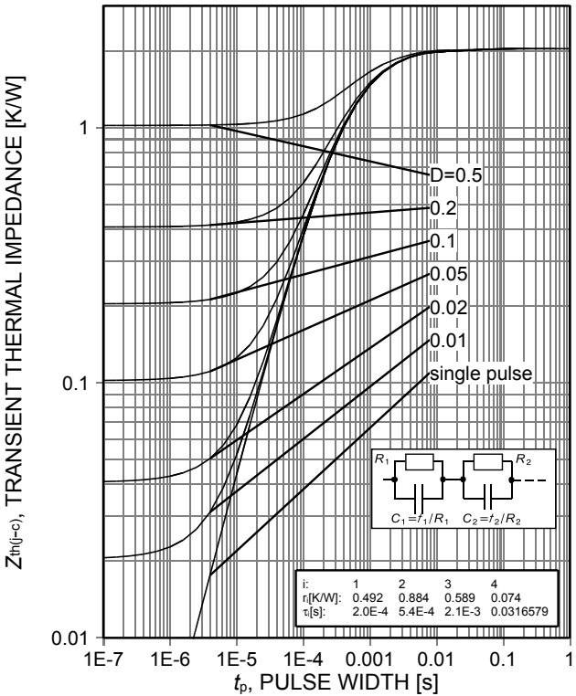
Figure 19. IGBT transient thermal impedance 1) ( D = t_p/T )
