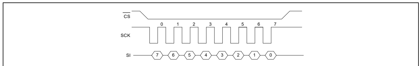
Figure 5 SPI Mode 3
