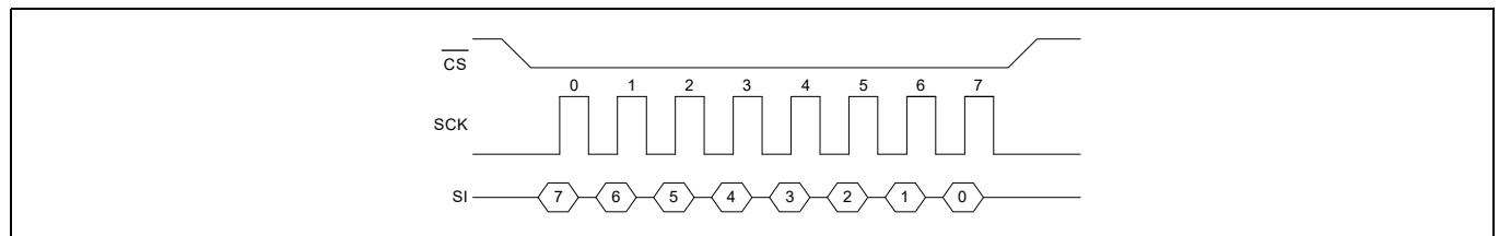
Figure 4 SPI Mode 0
