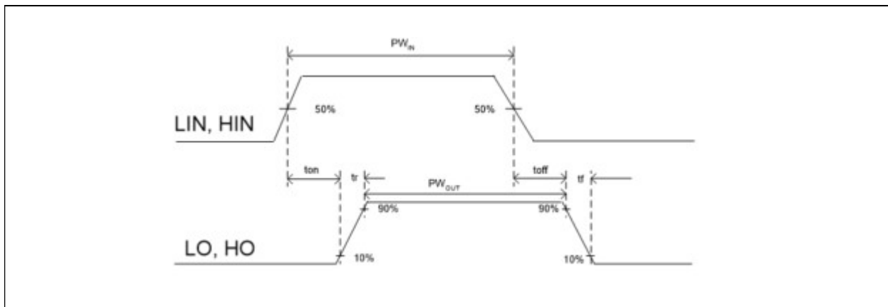
Figure 6 Switching timing diagram
