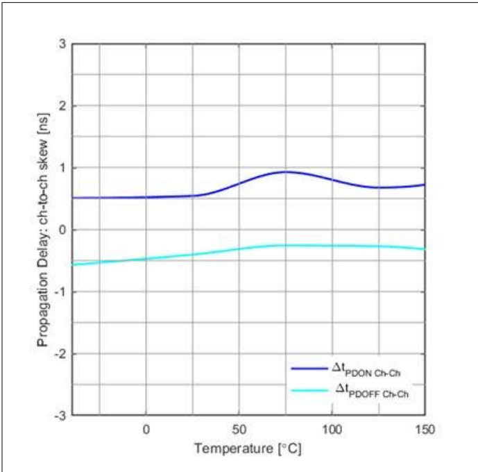
Figure 16 \Delta t_{PDON, Ch-Ch} & \Delta t_{PDOFF, Ch-Ch} vs. temperature
