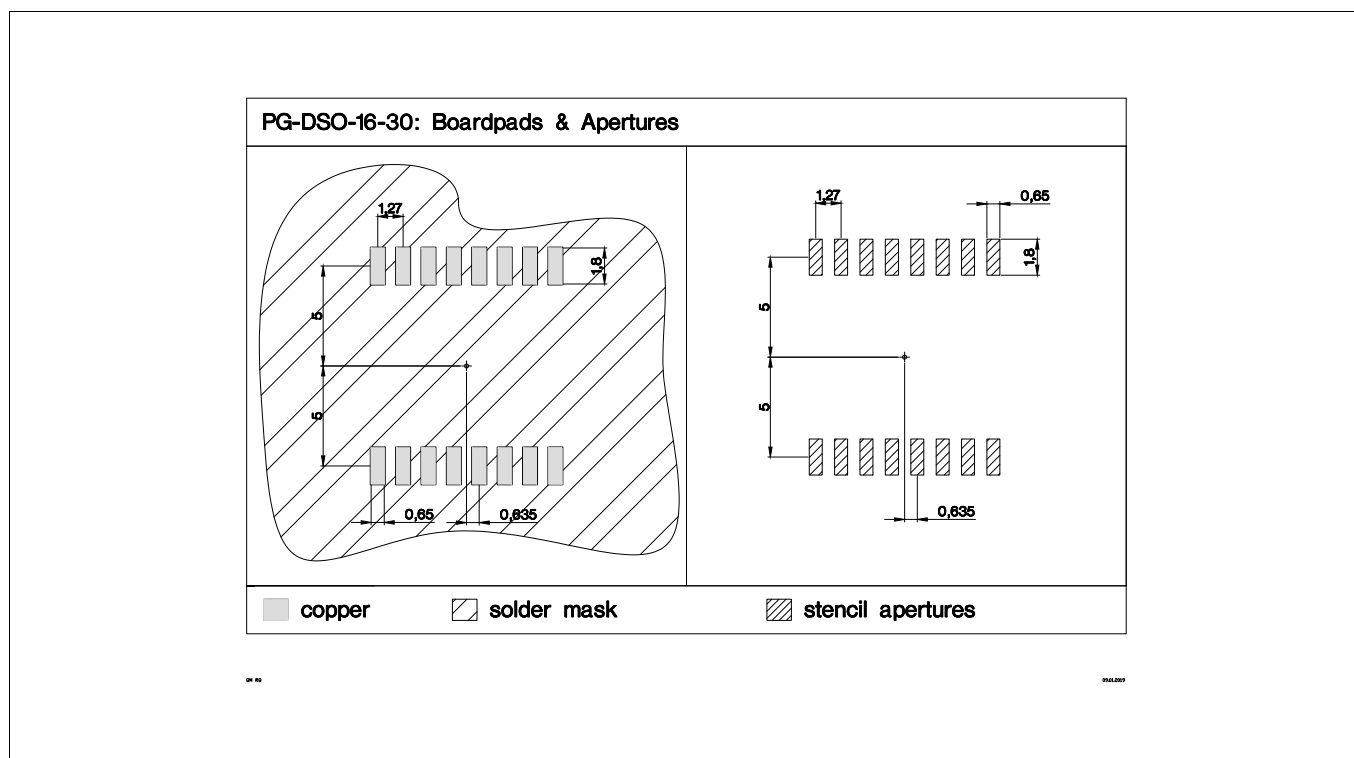
Figure 21 PG-DSO-16-30 footprint
