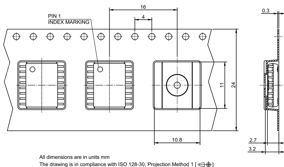
Figure 20 PG-DSO-16-30 packaging
