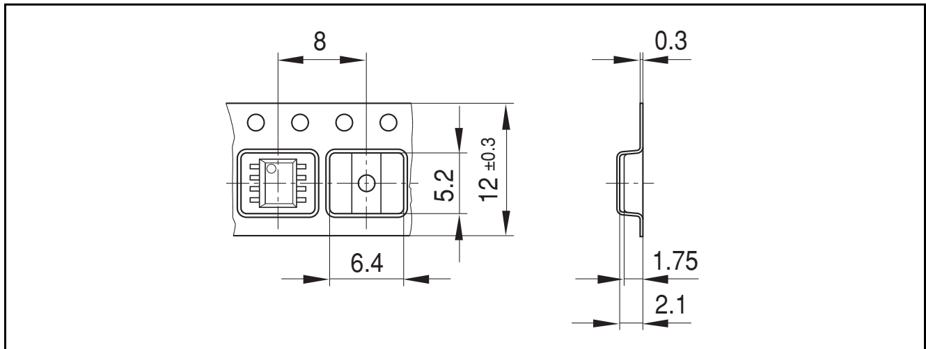
Figure 8-3 PG-DSO-8-60 packaging
