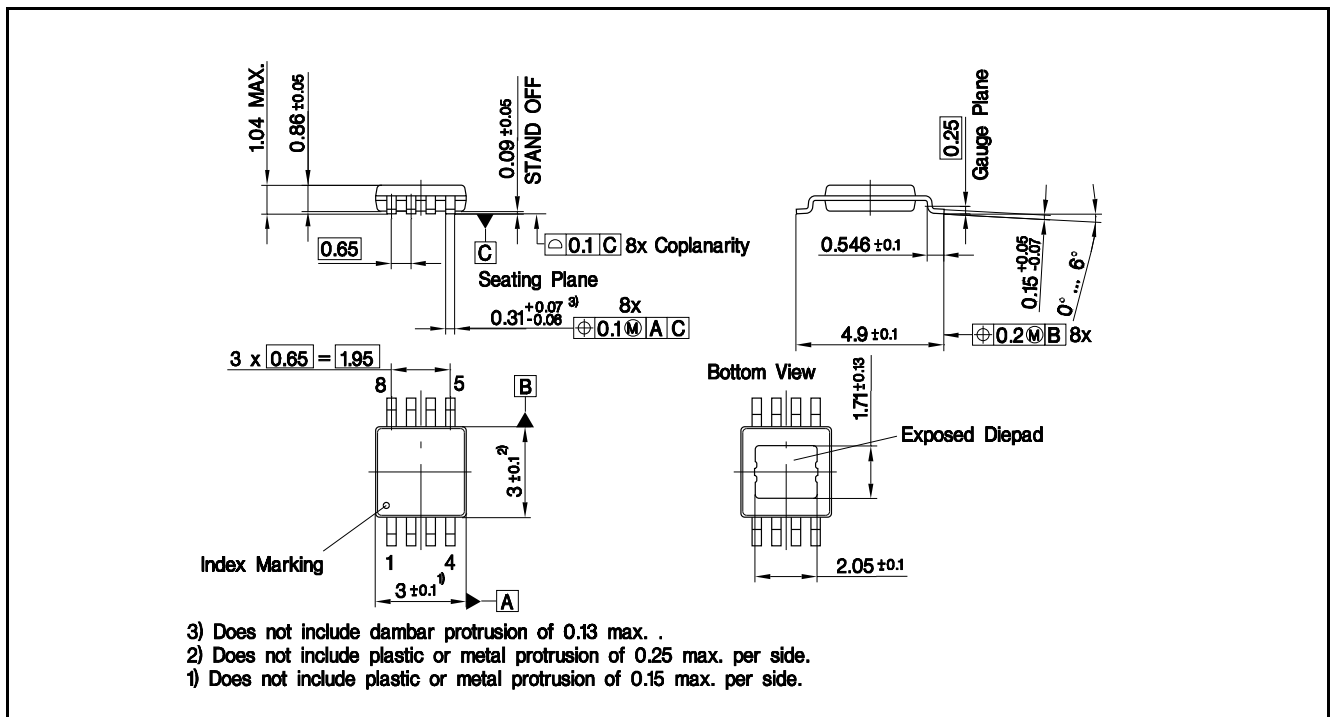
Figure 8-4 PG-TSSOP-8-1 outline
