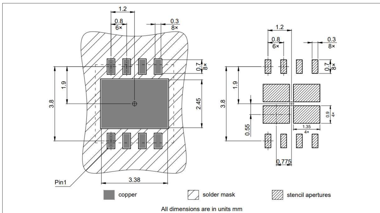
Figure 31 PG-VDSON-8-5 footprint dimensions
