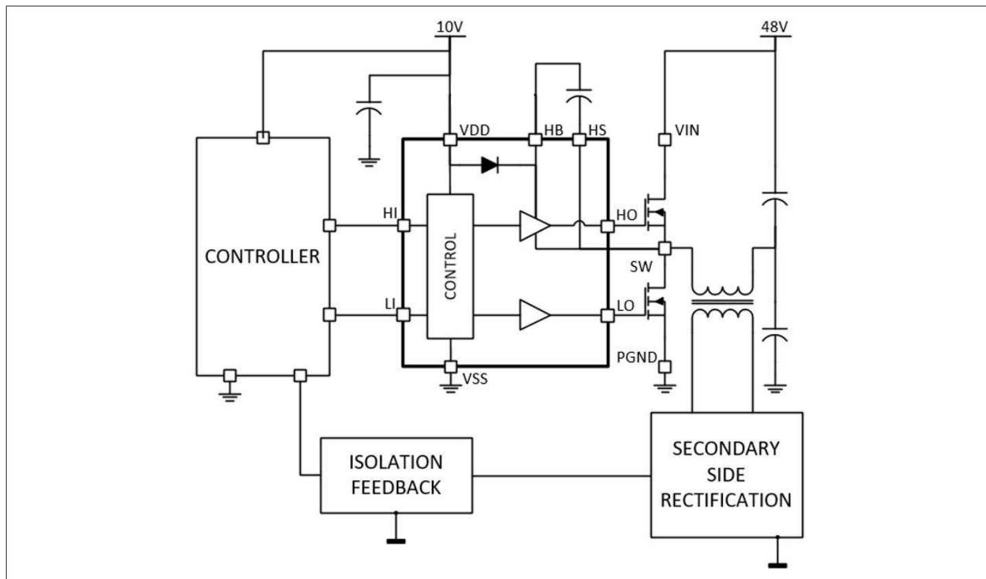
Figure 26 Typical application - primary side half-bridge
