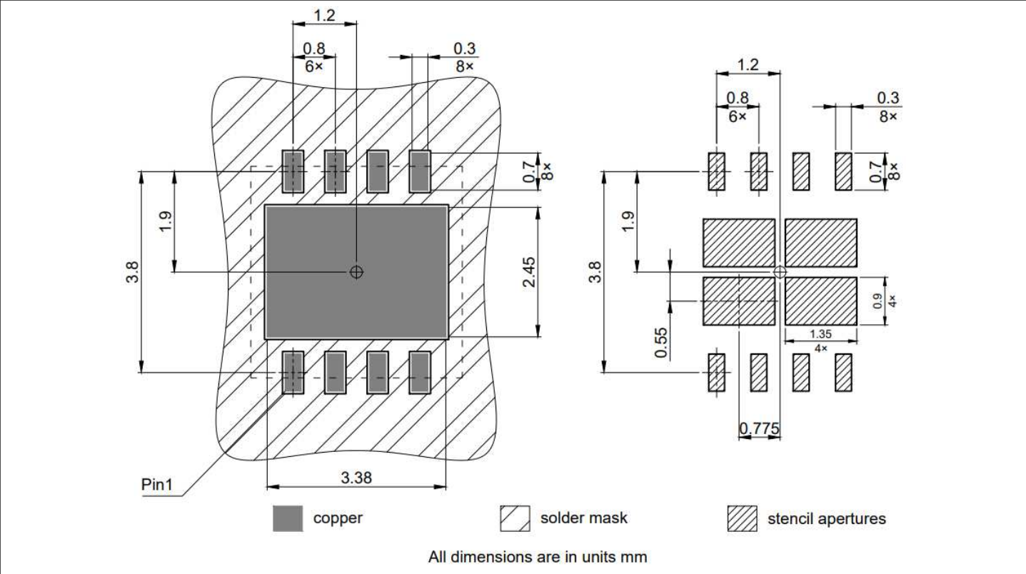
Figure 31 PG-VDSO8-5 footprint dimensions
