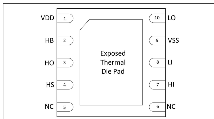
Figure 2 VDSO8-10 4 mm x 4 mm, Top transparent view
