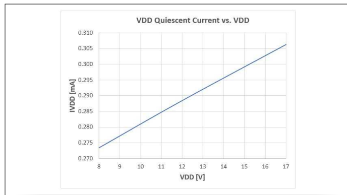
Figure 13 VDD quiescent current vs. VDD
