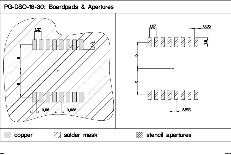
Figure 21 PG-DSO-16-30 footprint
