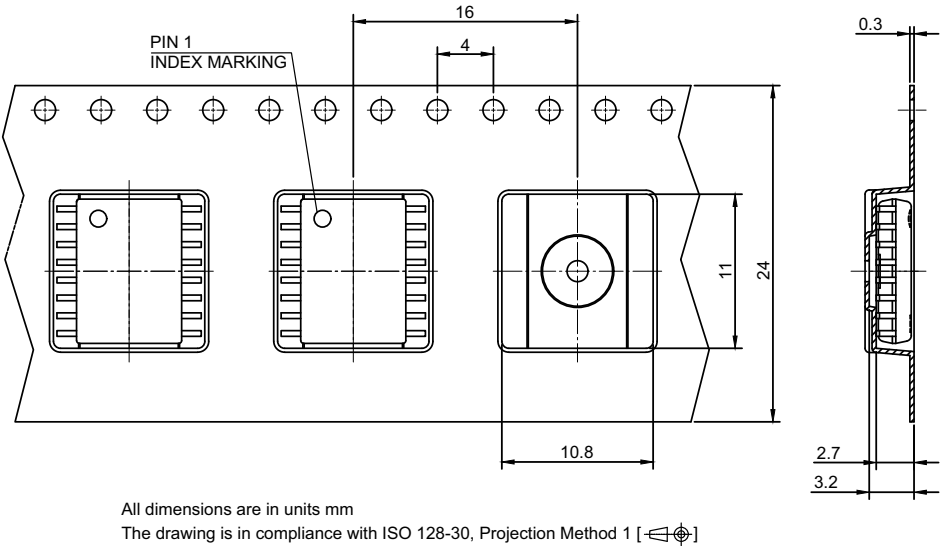
Figure 22 PG-DSO-16-30 packaging
