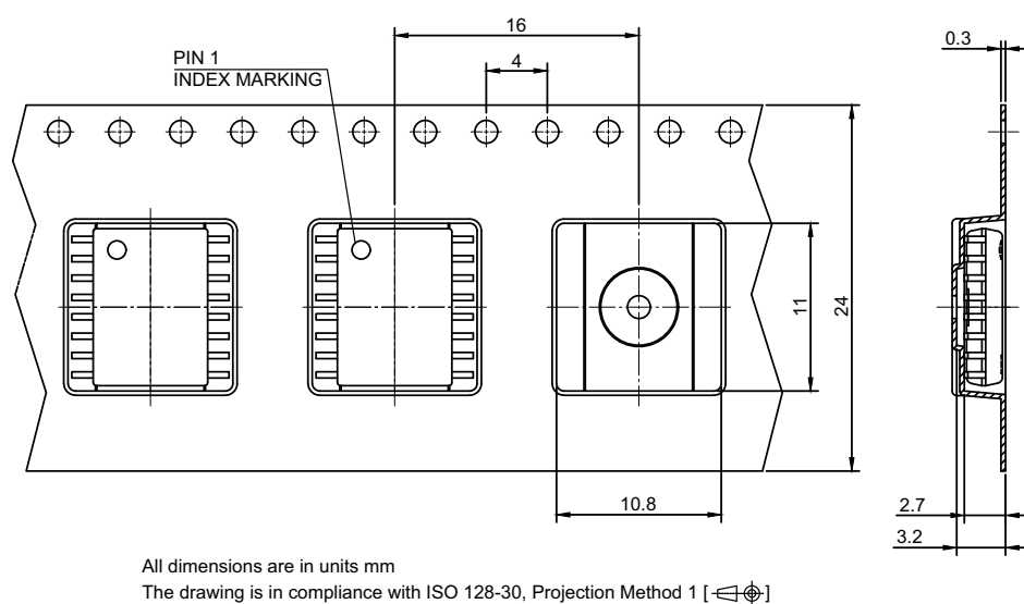
Figure 22 PG-DSO-16-30 packaging
