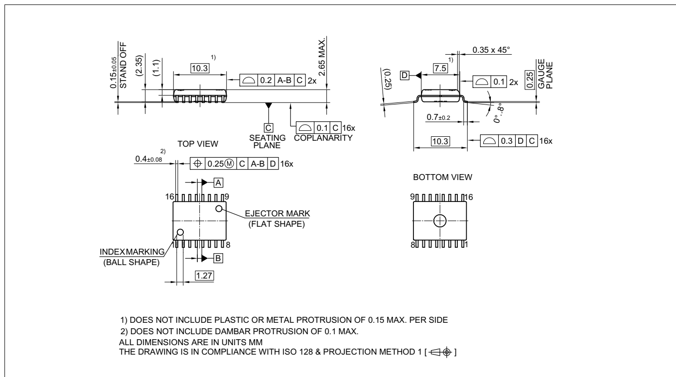
Figure 20 PG-DSO-16-30 outline
