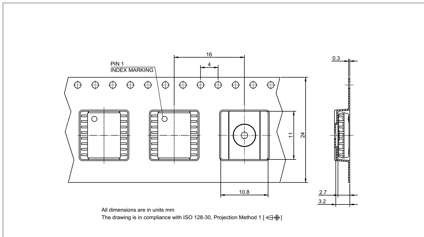
Figure 22 PG-DSO-16-30 packaging
