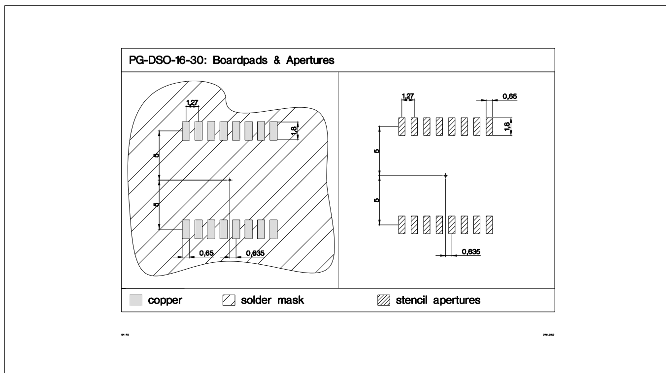
Figure 21 PG-DSO-16-30 footprint
