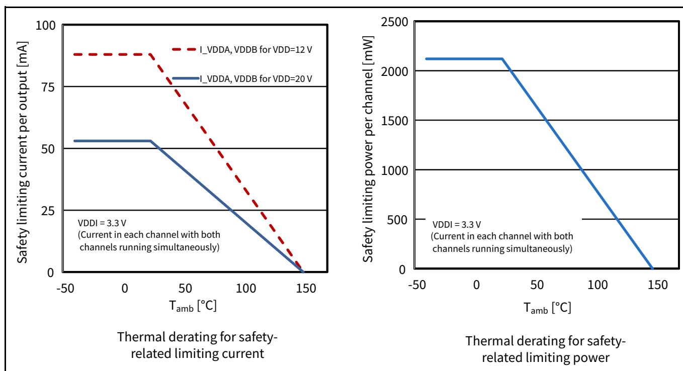
Figure 16 Thermal derating curves
