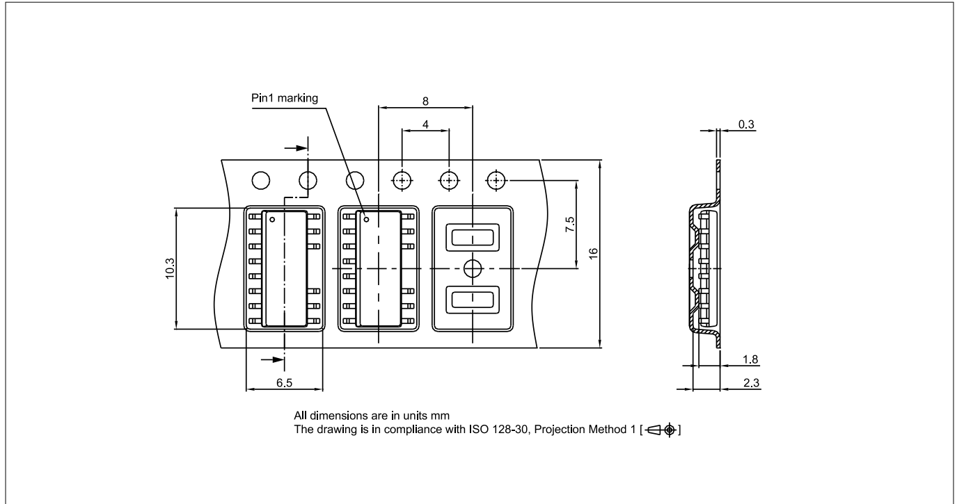
Figure 26 DSO14-150mil packing
