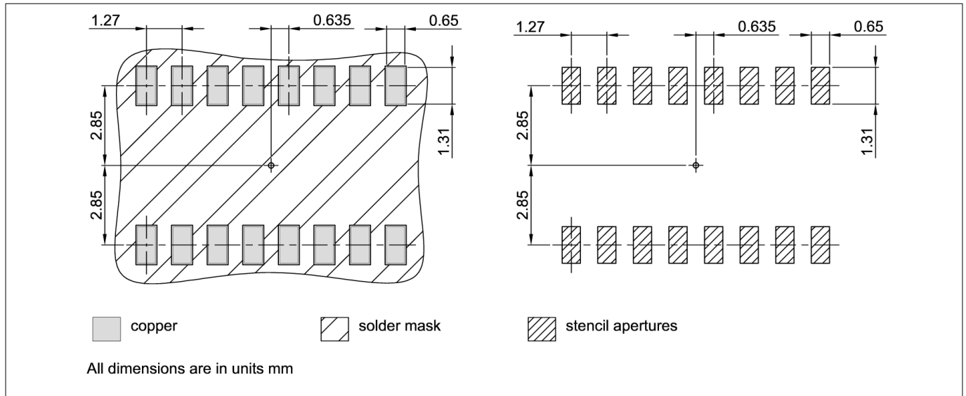
Figure 22 DSO16-150mil footprint
