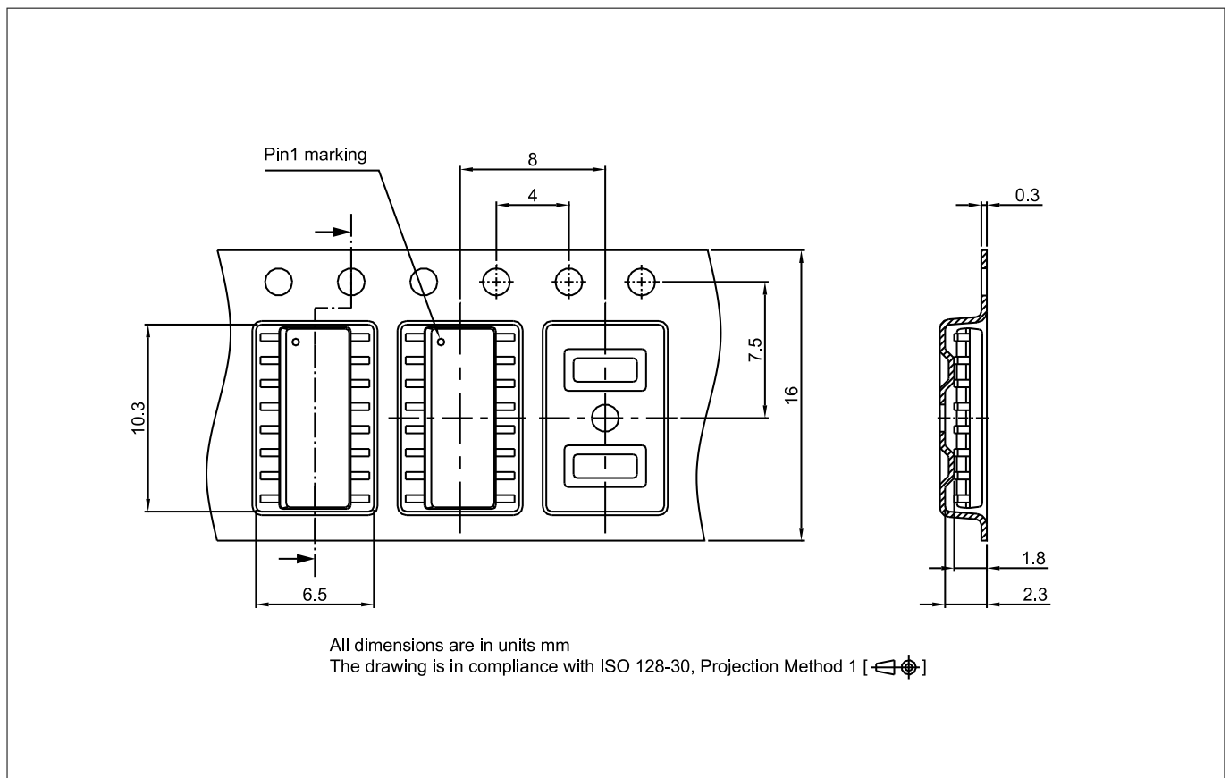
Figure 23 DSO16-150mil packing
