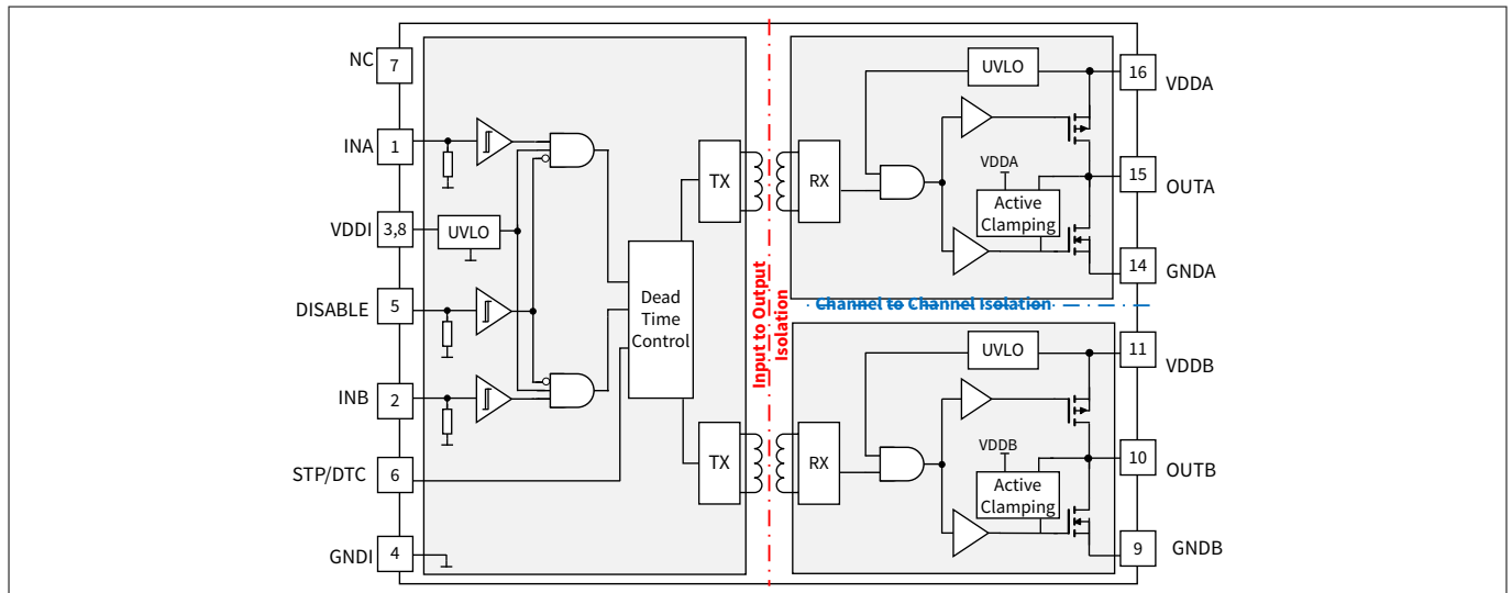
Figure 3 Block diagram
