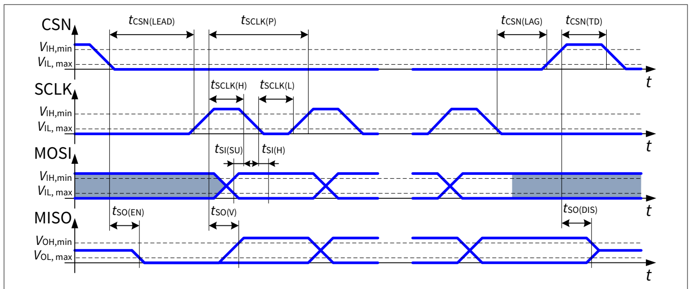
Figure 10 SPI timings
