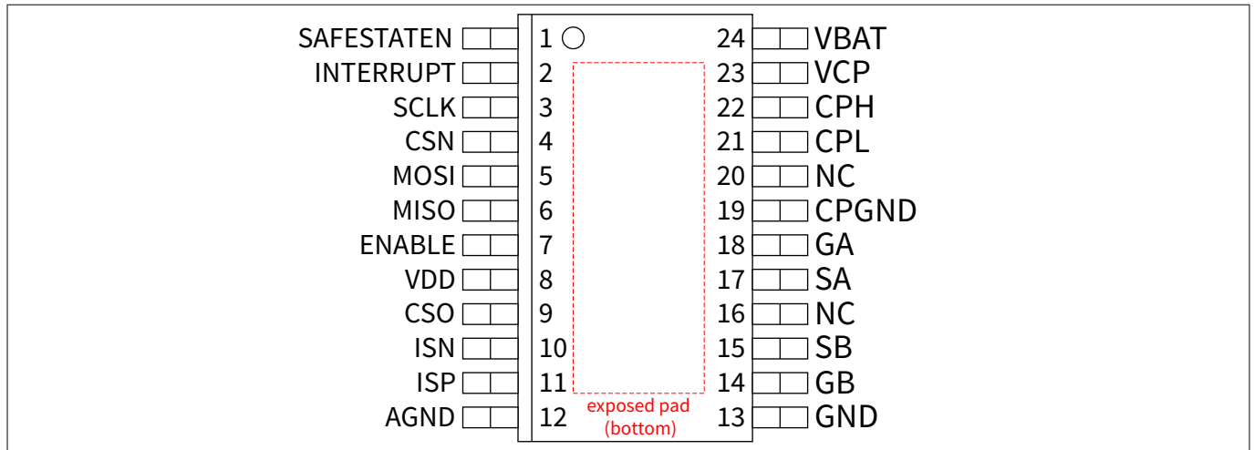
Figure 3 Pin assignment
