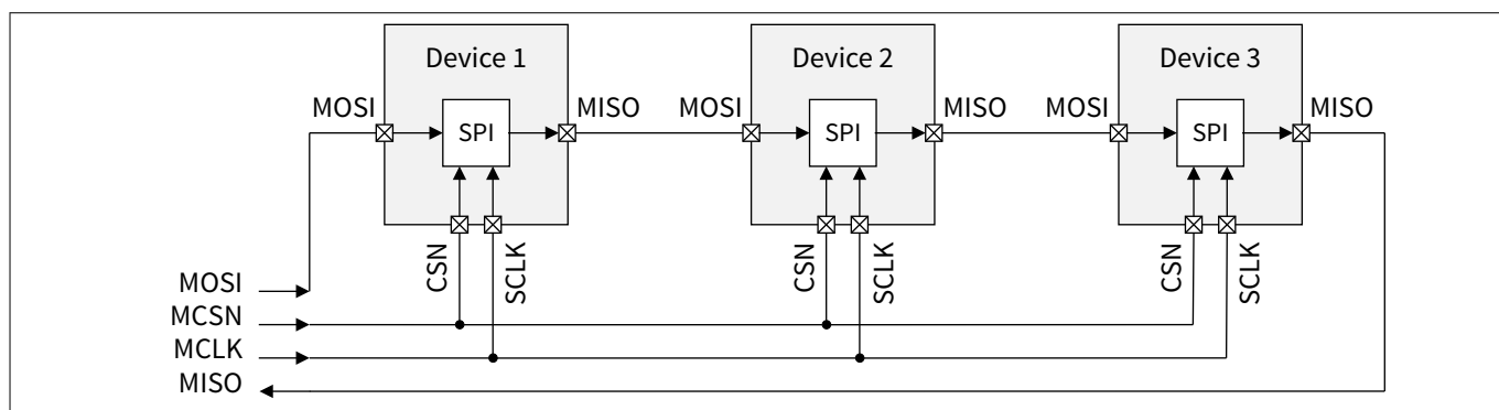
Figure 11 Daisy chain capability
