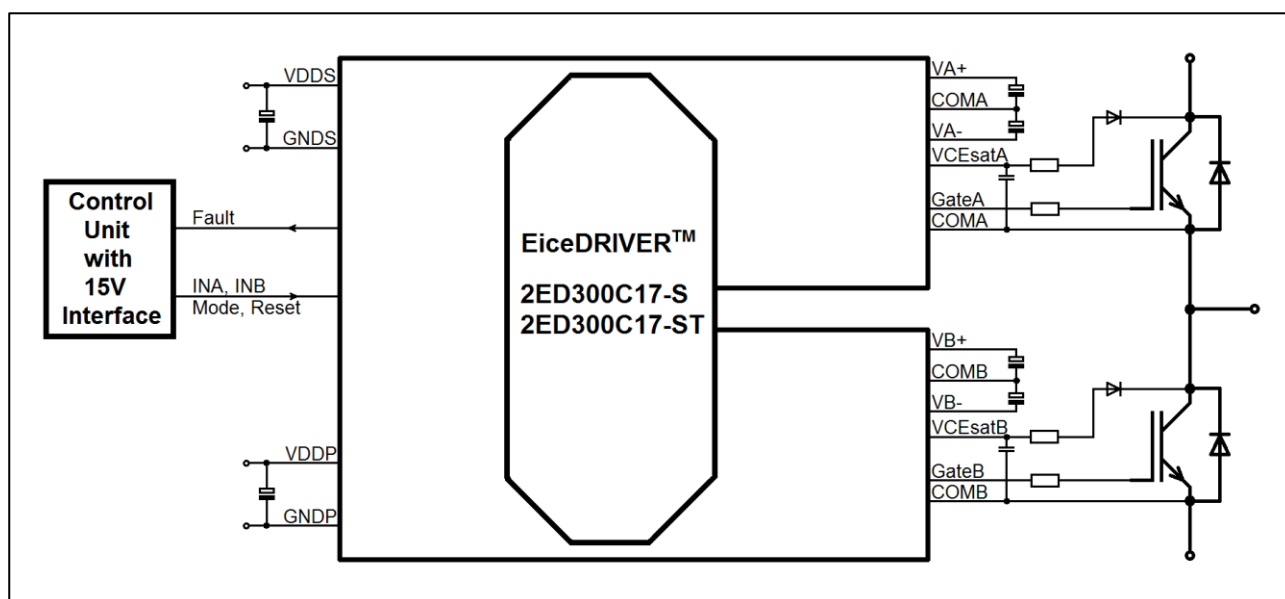
Figure 1: Basic schematic for driver setup
