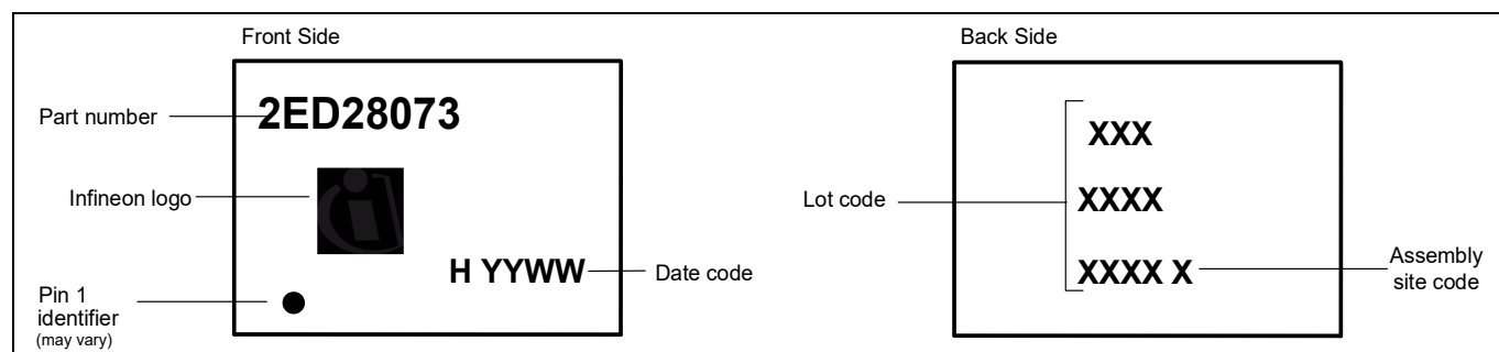
Figure 28 Marking information PG-DSO-8 (2ED28073J06F)
