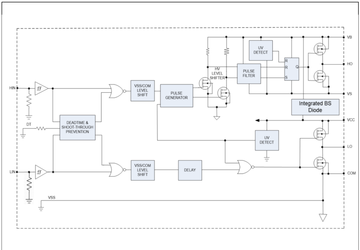
Figure 2 Block diagram
