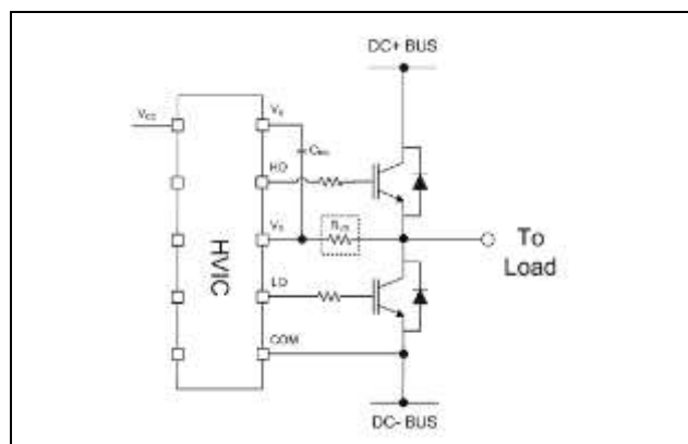
Figure 19 Resistor between the V_S pin and the switch node
