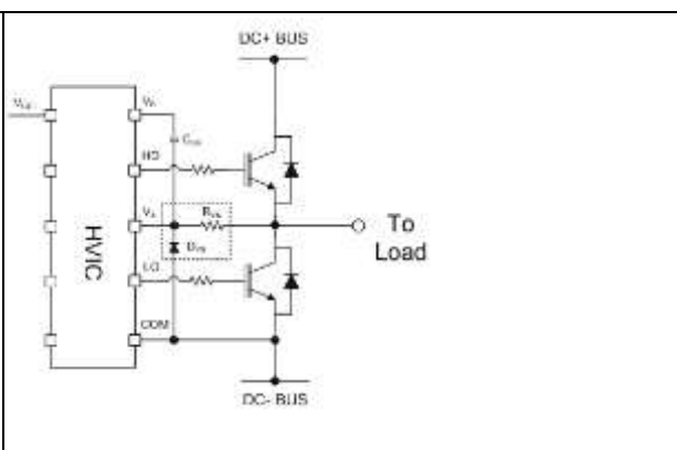
Figure 20 Clamping diode between COM and V_S
