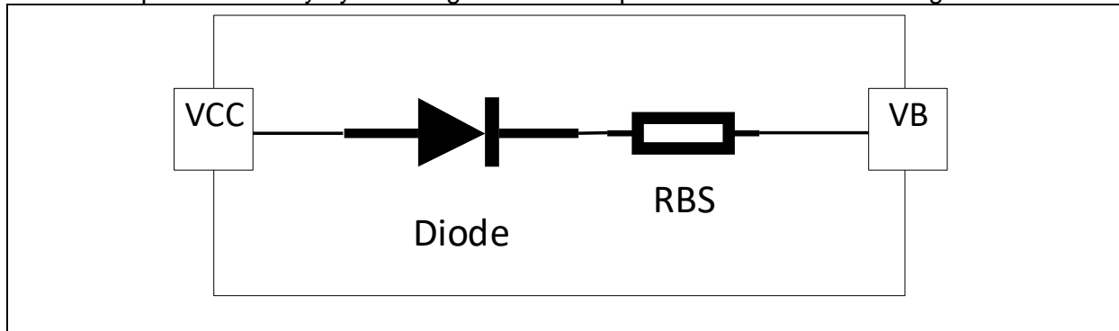
Figure 13 2ED2748S01G with integrated components
