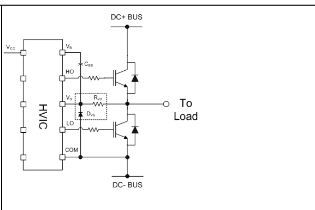
Figure 18 Clamping diode between COM and V_S
