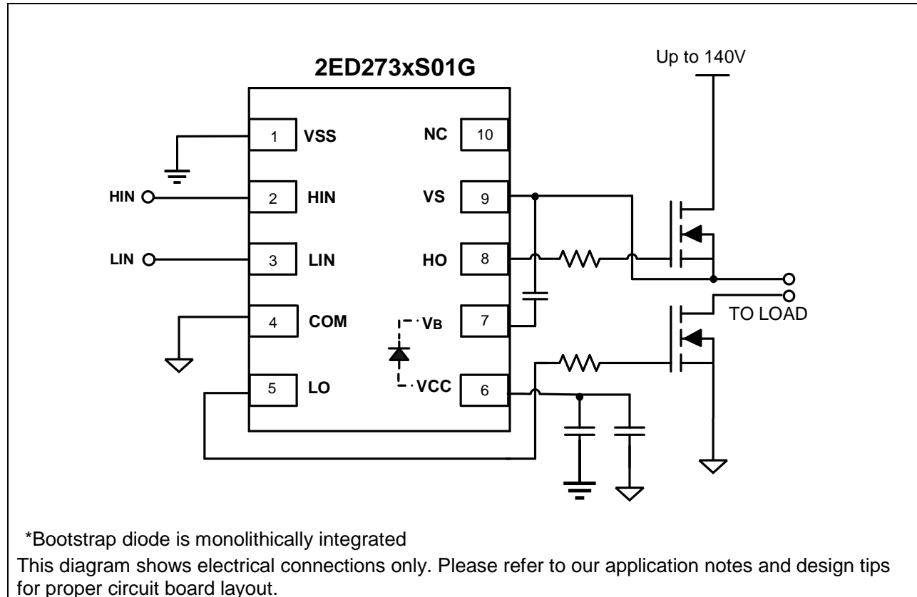
Figure 1 Typical application block diagram
