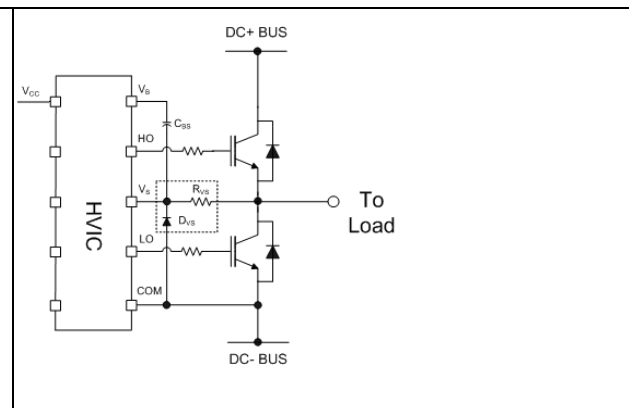
Figure 18 Clamping diode between COM and VS
