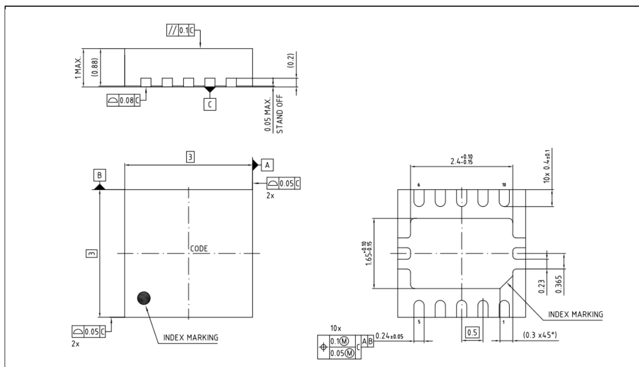
Figure 19 Target Package Dimensions: PG-VSON-10-5 (2ED2732S01G)
