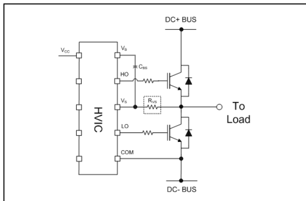
Figure 17 Resistor between the VS pin and the switch node
